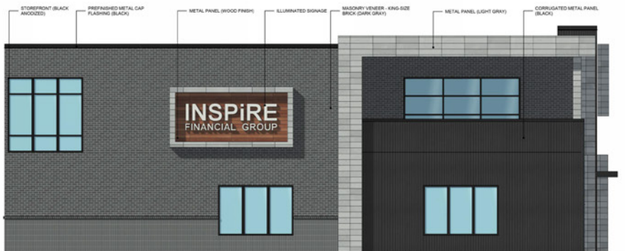
EAST ELEVATION
