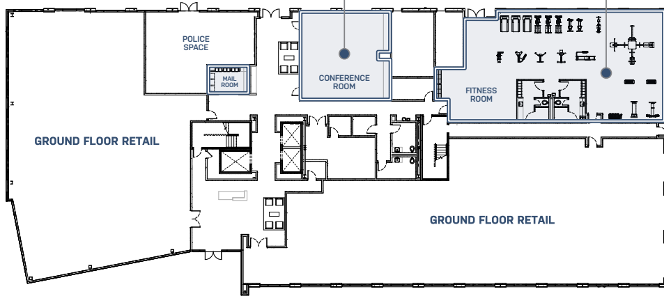
TRINITY MILLS STATION I LEVEL 1 · 15,300 SF
