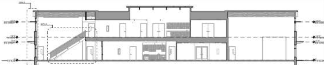
07 E-W Section @ Office
