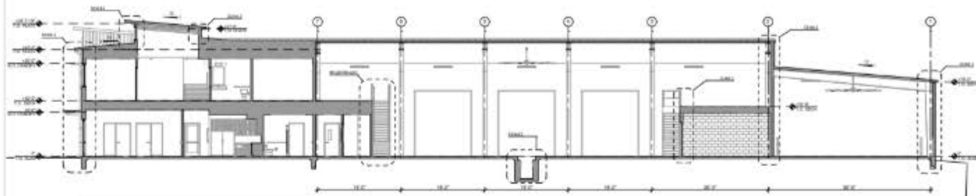
02 E-W Building Section @ Clearstory
