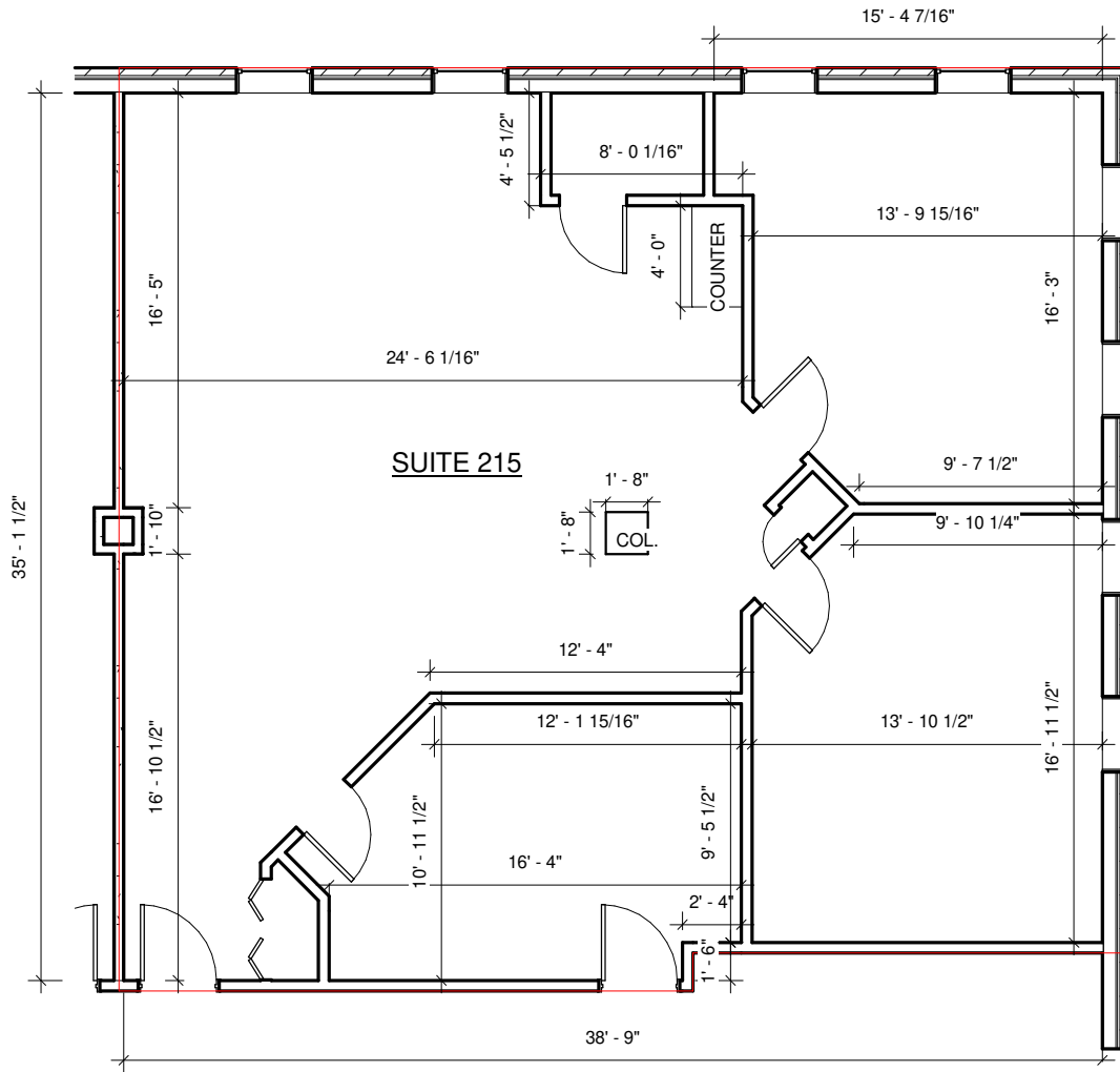
① Suite 215 1/8" = 1'-0"
