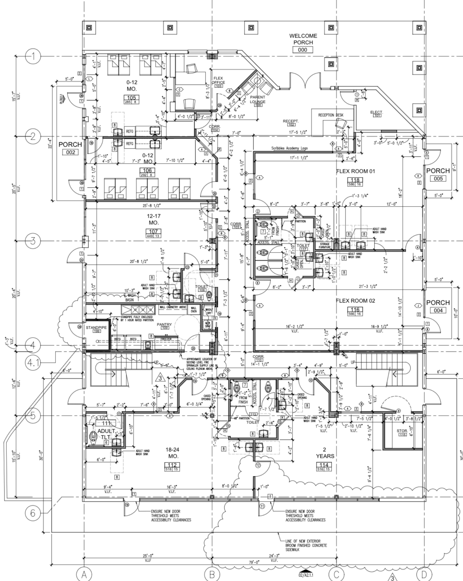
01 OVERALL FLOOR PLAN 3/16" = 1'-0"
