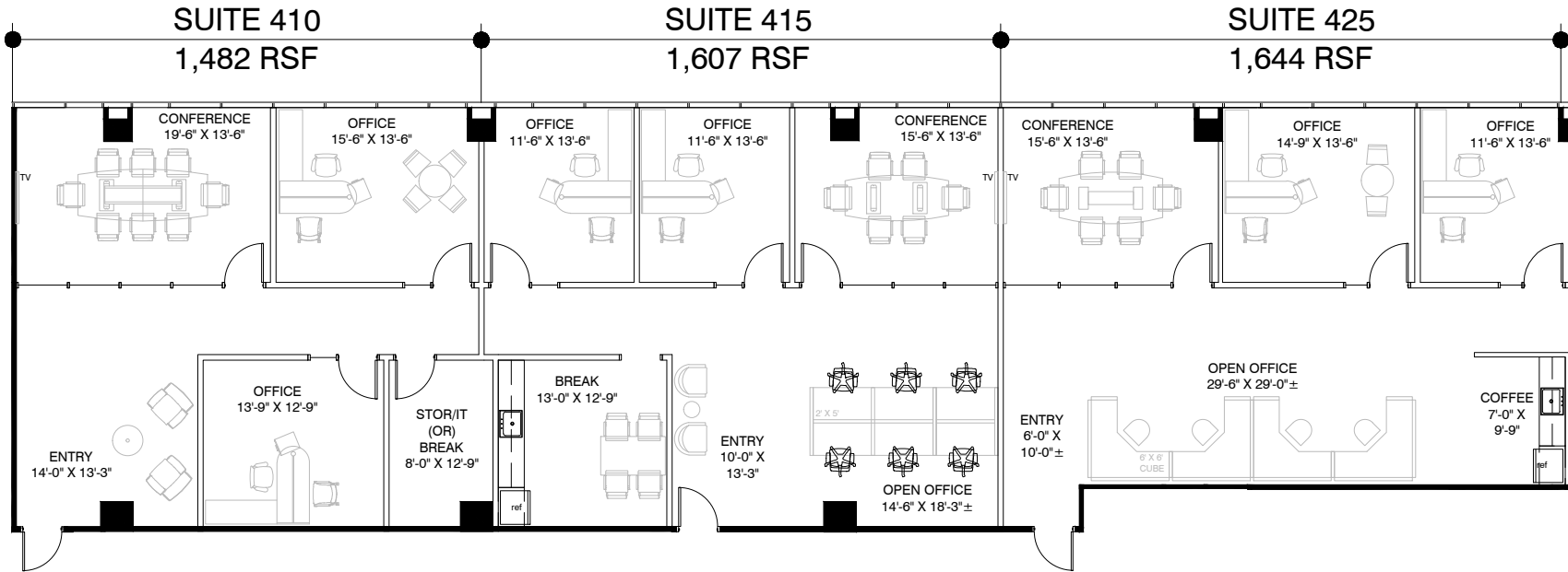
KEYPLAN - 4TH FLOOR
