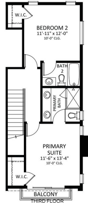
THIRD FLOOR
