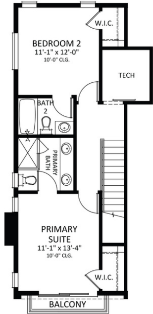
THIRD FLOOR
