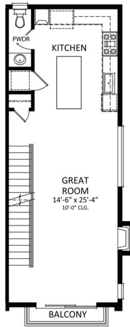
SECOND FLOOR
