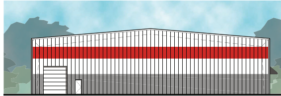
SOUTH ELEVATION
