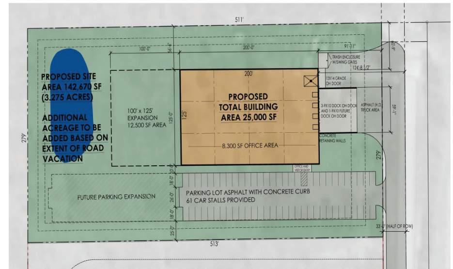
SITE STUDY - OPTION B Scale: 1" = 40'-0"
