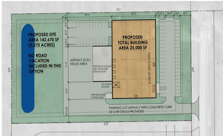
SITE STUDY - OPTION A Scale: 1" = 40'-0"
