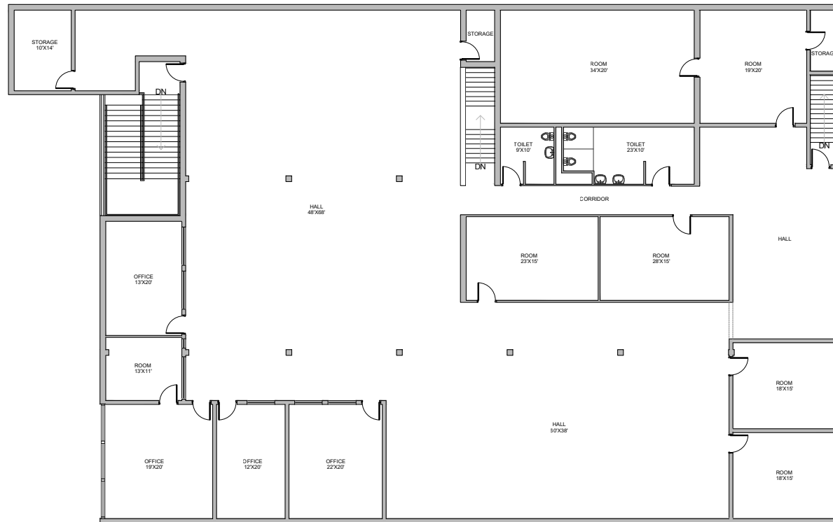
1 SECOND FLOOR PLAN SCALE = 1/4" = 1'-0"
