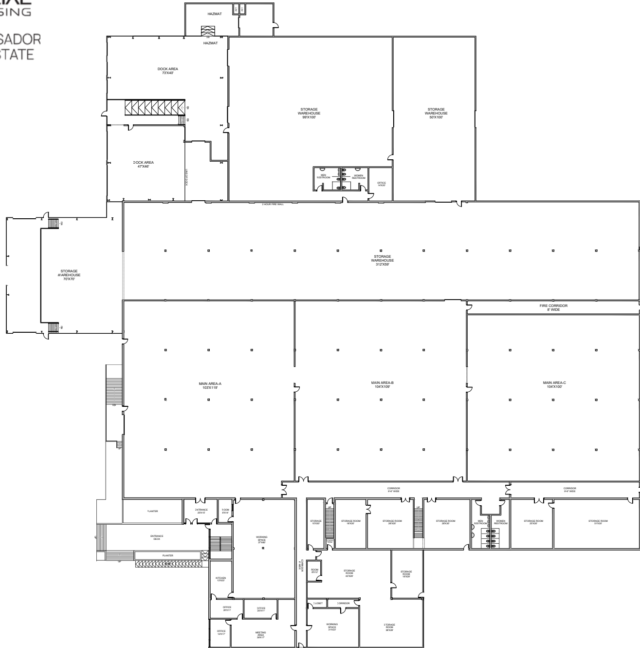
① FIRST FLOOR PLAN SCALE: 1/8" = 1'-0"
