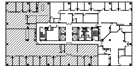
KEYPLAN - 3RD FLOOR
