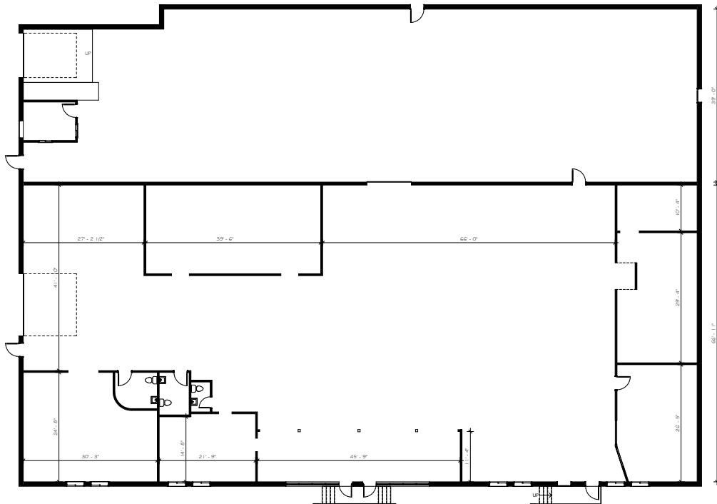
1 FIRST FLOOR 1/8" = 1'-0"
