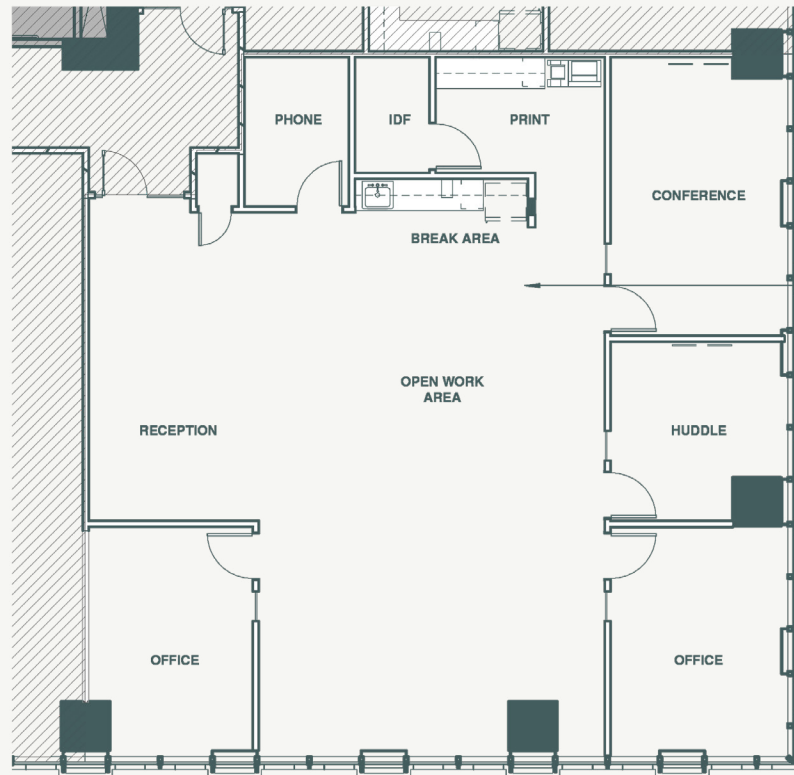
2 Level 5- Marketing Suite D 1/8" = 1'-0"
