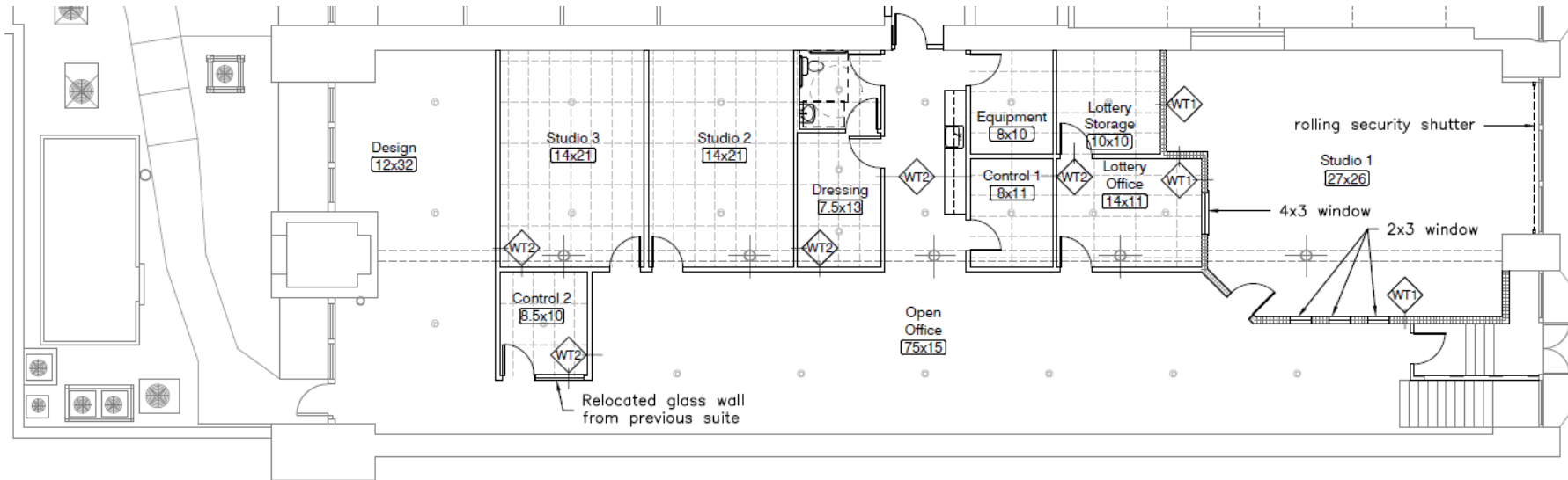
1st FLOOR PLAN 3/32" = 1'-0"
