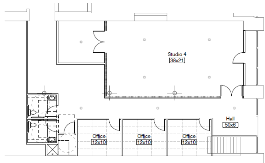
1st FLOOR PLAN 3/32" = 1'-0"
