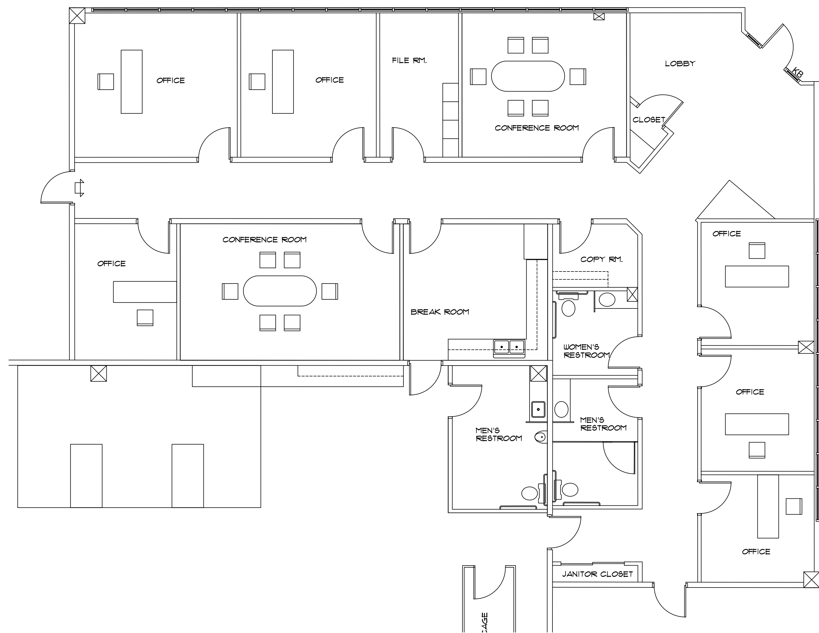
2 ENLARGED OFFICE AREA A2.0 3/16" = 1' - 0" SCALE WITH EQUIPMENT
