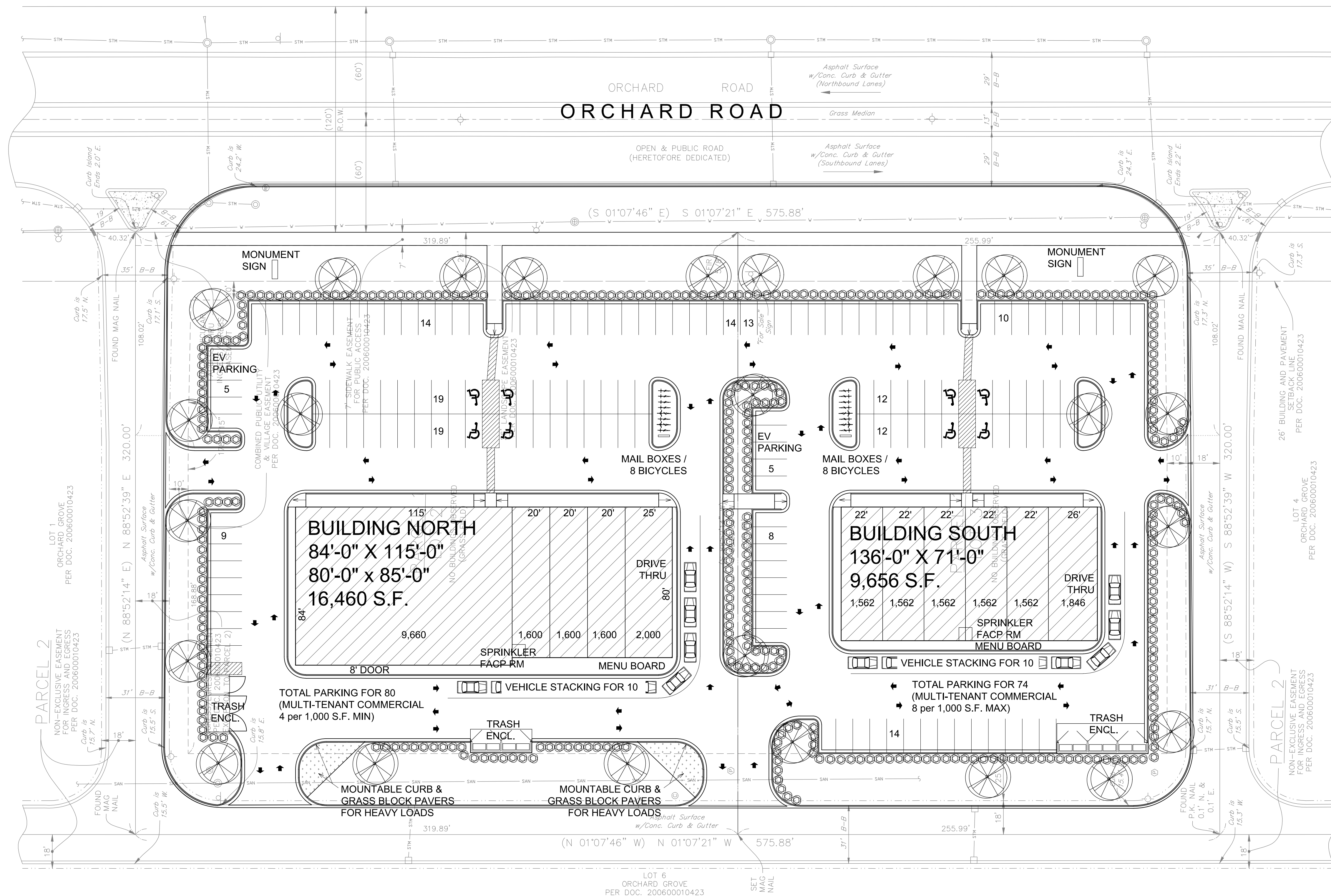
1 ARCHITECTURAL SITE PLAN 1/30" = 1'-0"
