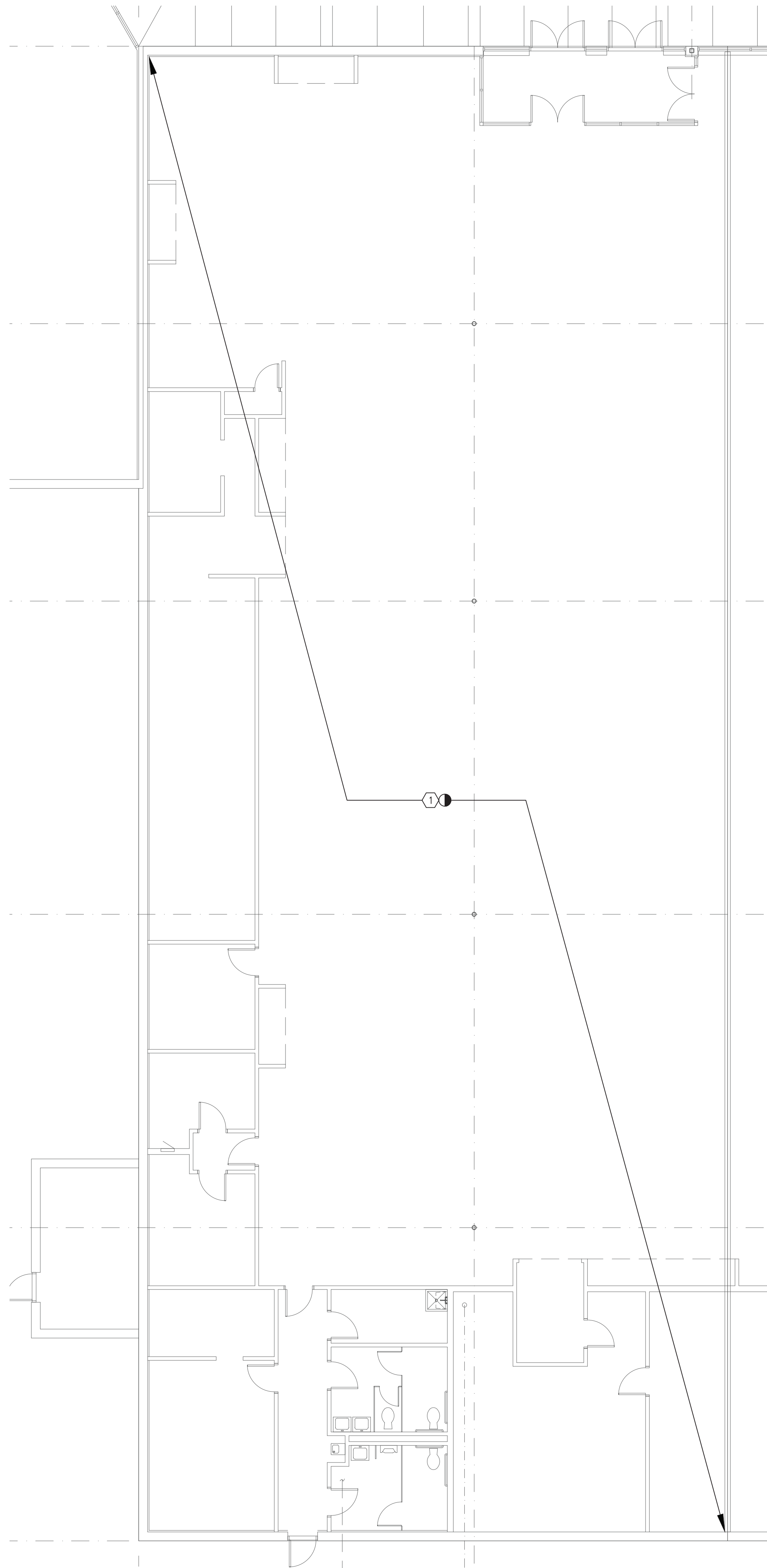
1 FIRE PROTECTION DEMOLITION PLAN SCALE: 1/8" = 1'-0"
