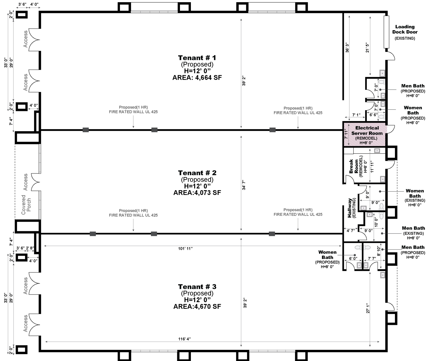
FLOOR PLAN - 410 S STATE RD 7, ROYAL PALM BEACH, FL 33414
