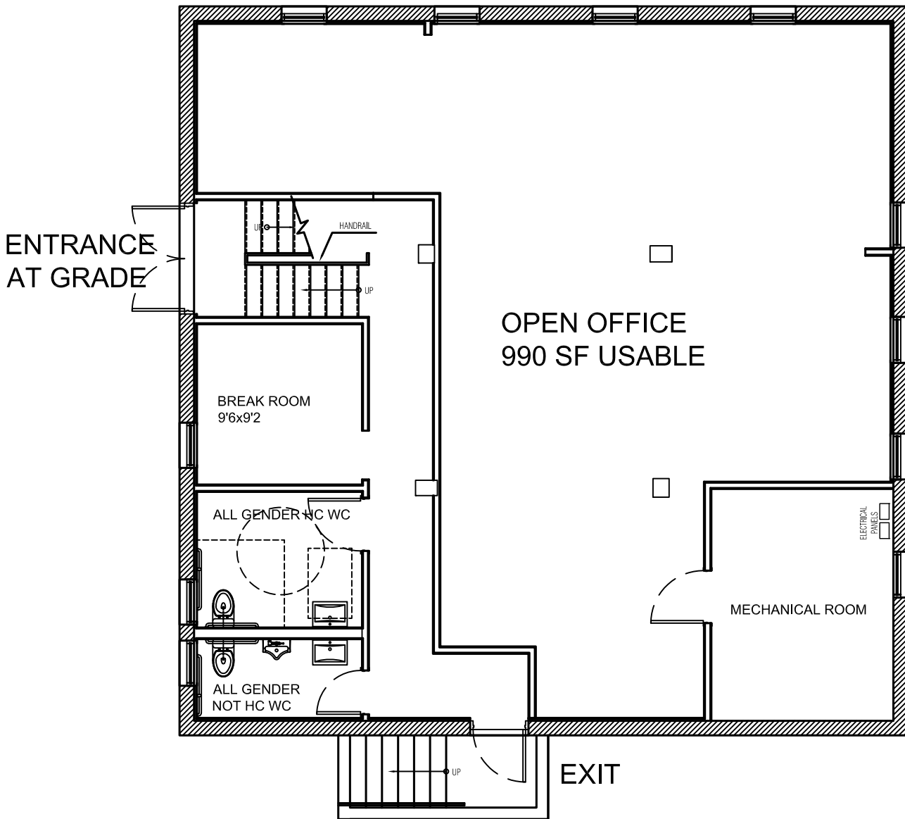
LOWER LEVEL FLOOR PLAN (HALF LEVEL DOWN)
