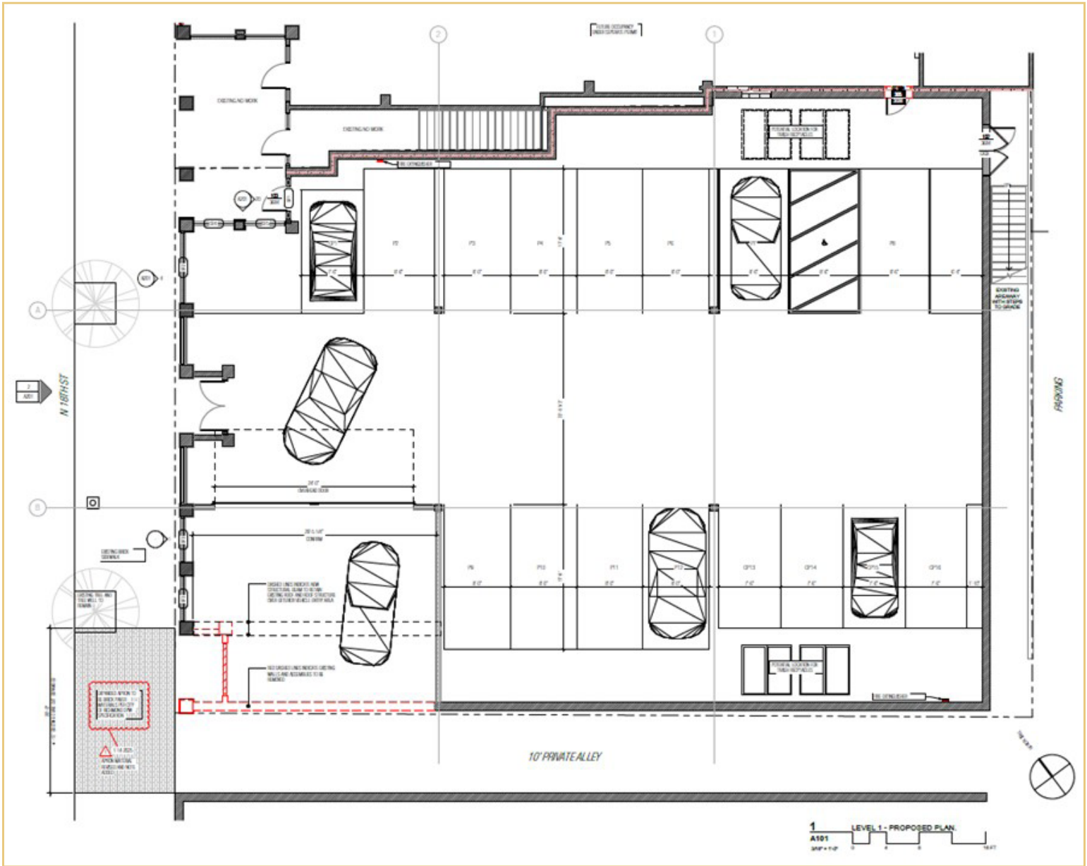
Parking Garage Plan
