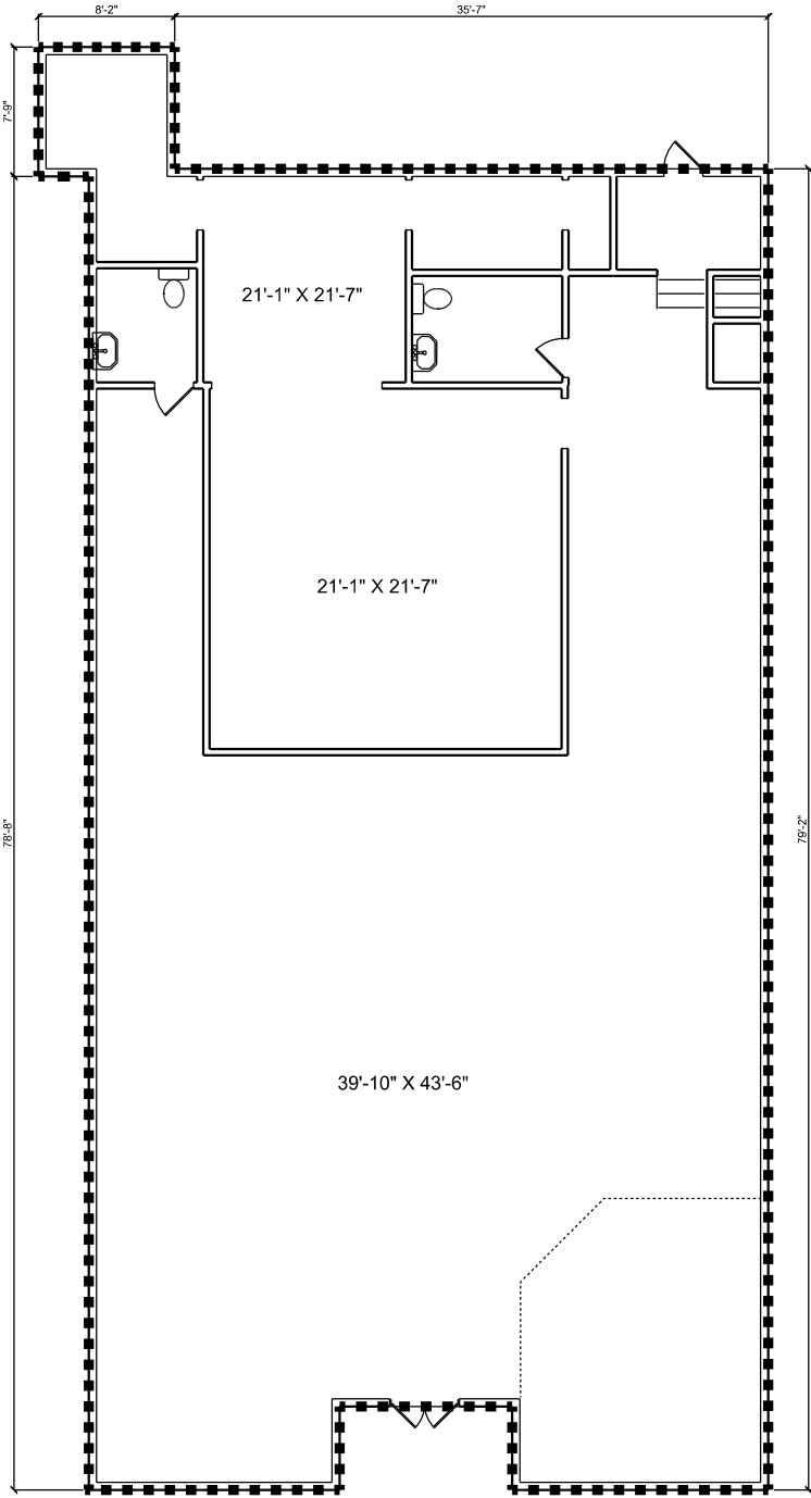
1ST FLOOR
