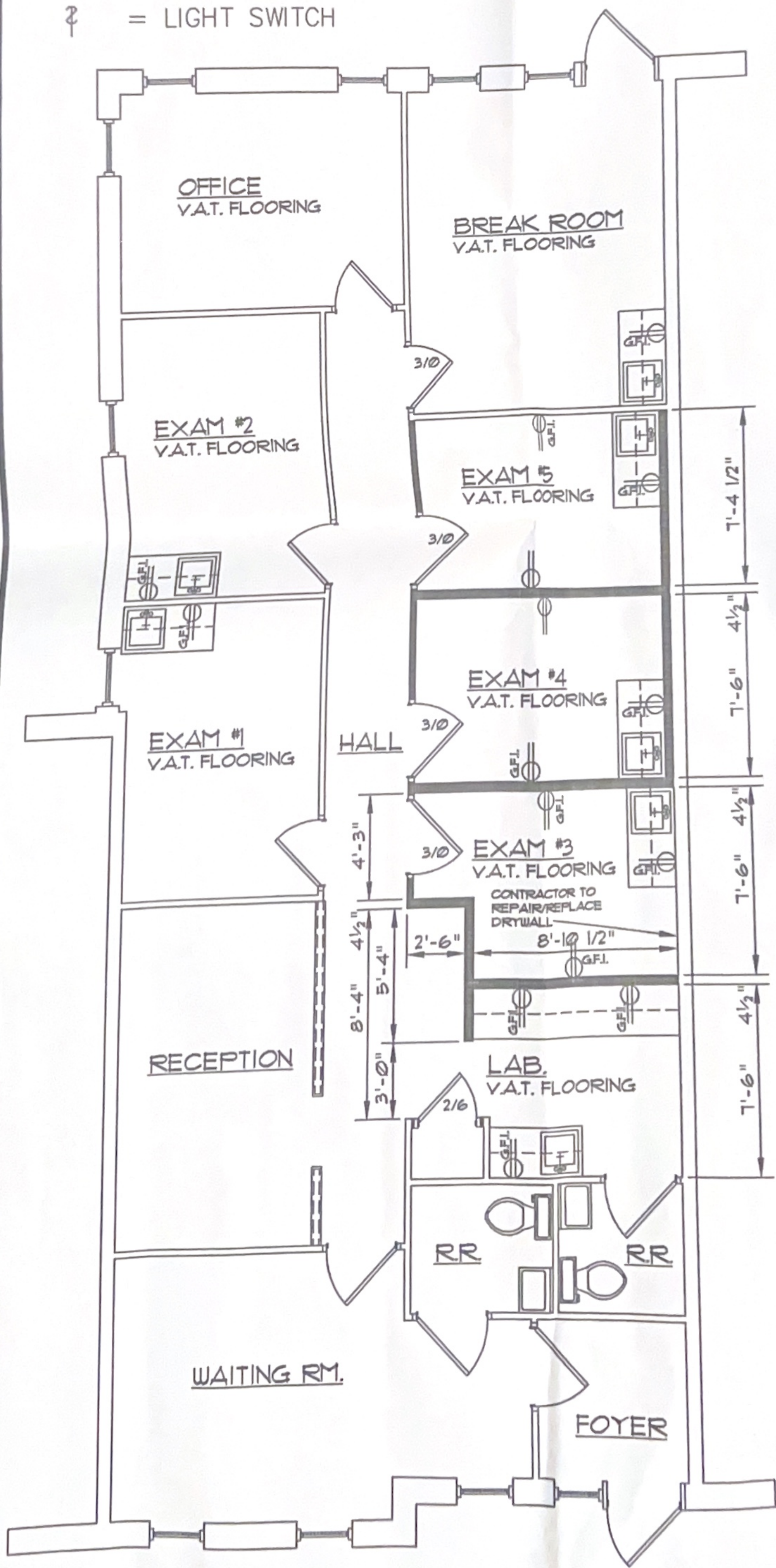
FLOOR PLAN SCALE = 1/4" = 1'-0"
