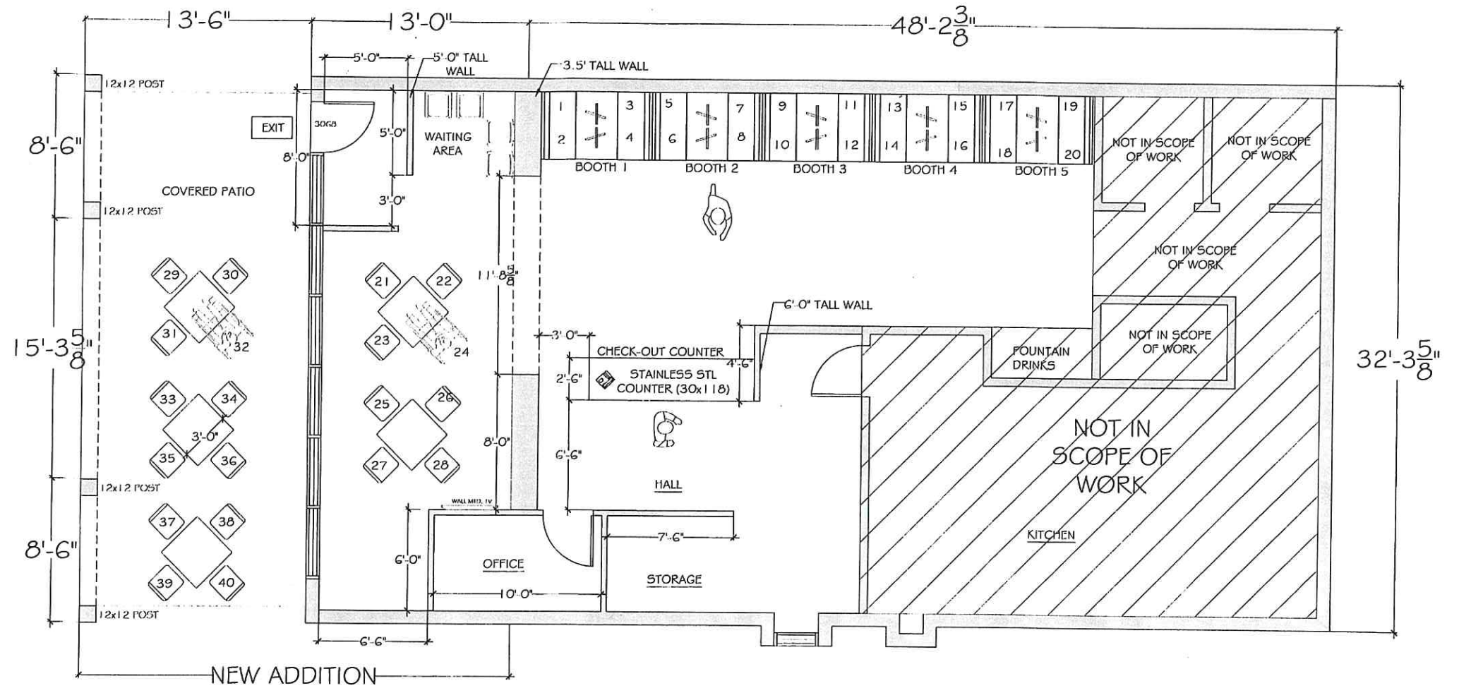
1 PROPOSED FLOOR PLAN SCALE: \frac{1}{4}" = 1' 0"
