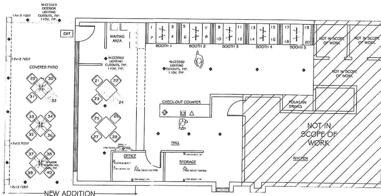
1 ELECTRICAL PLAN SCALE: 1/4" = 1'-0"
