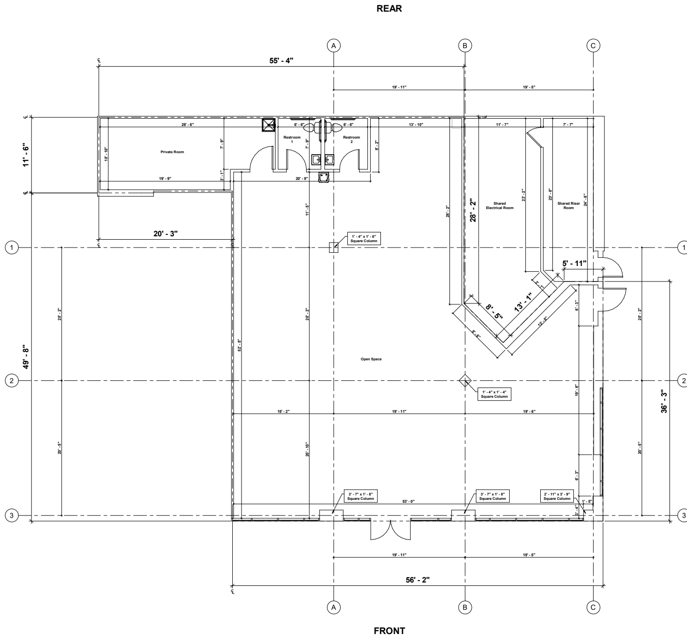
A1 MAIN FLOOR
