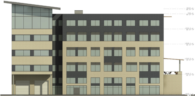
North Elevation
