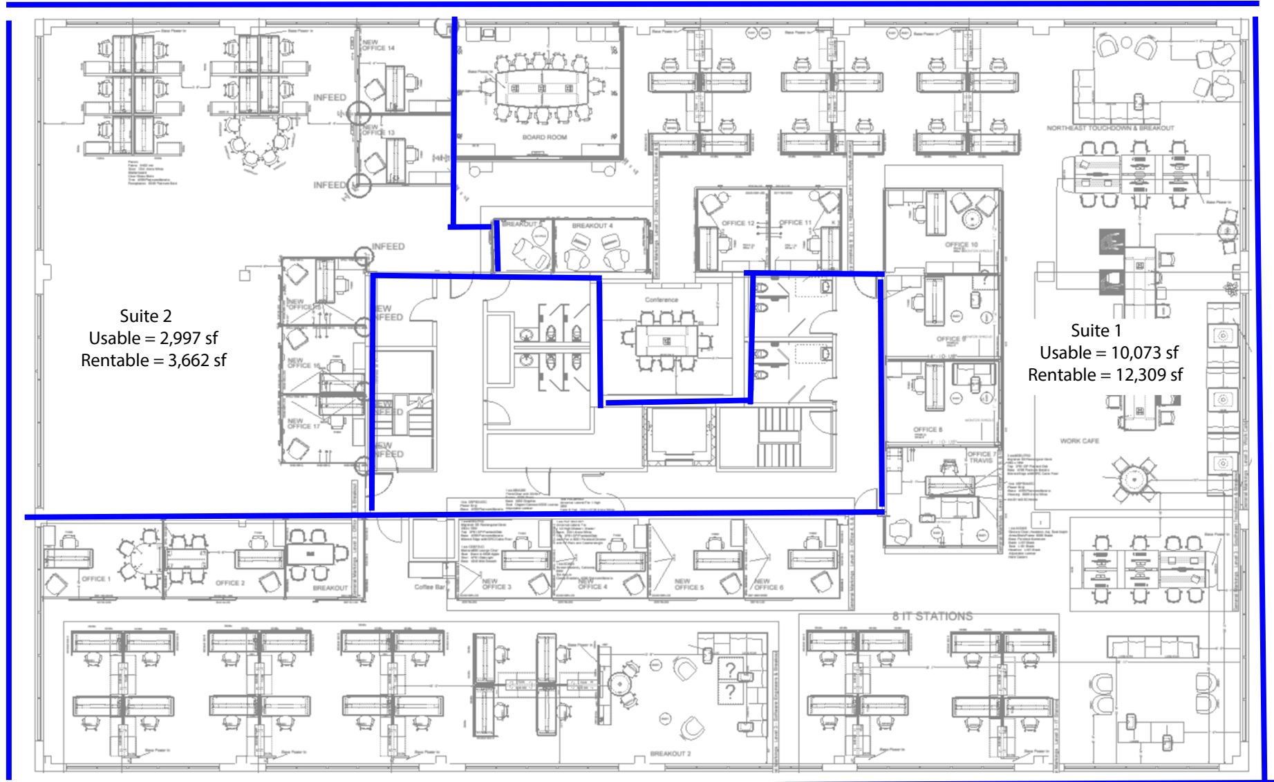
3rd Floor - EXISTING
