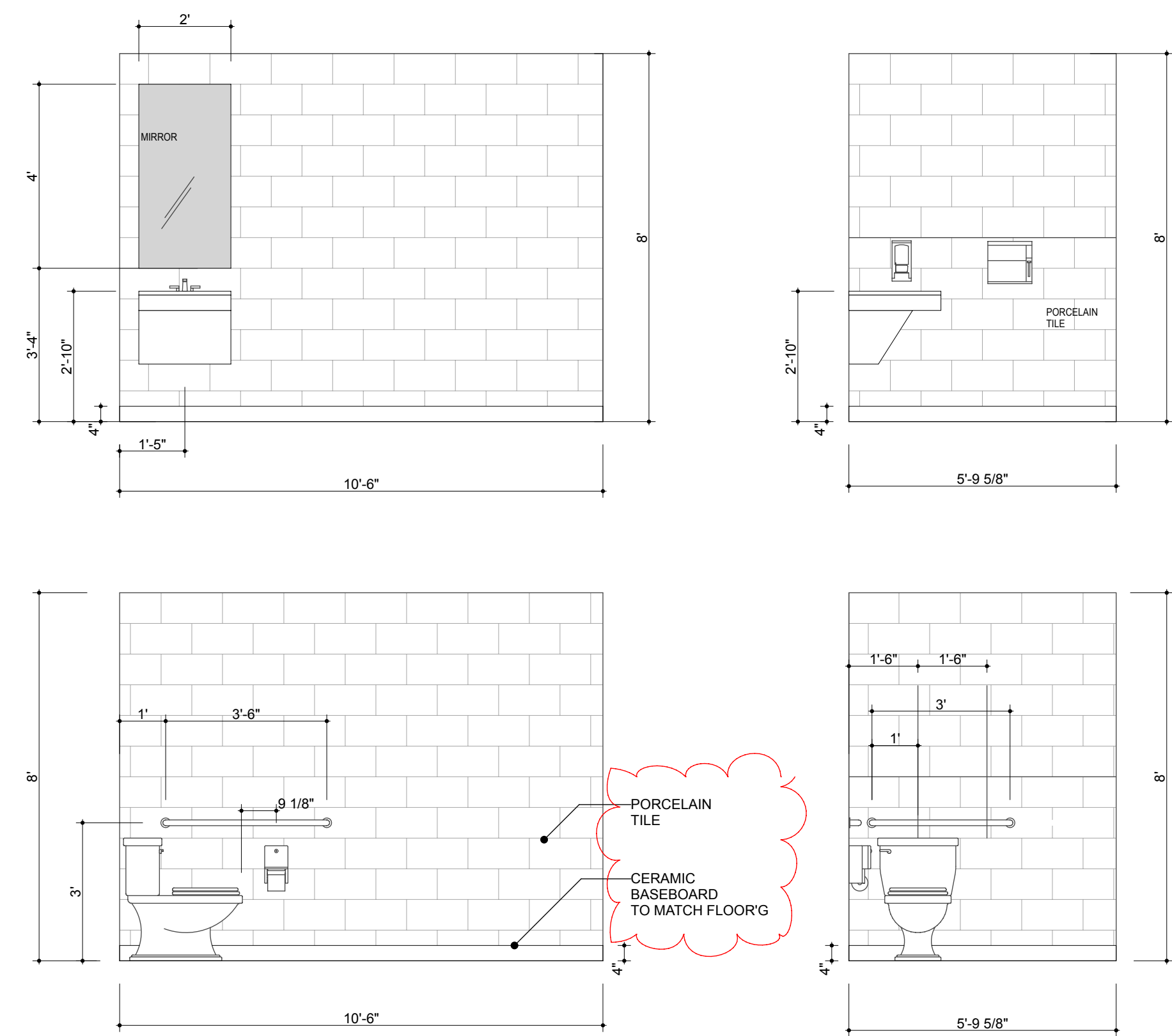
ADA typical bathroom elevations scale: 3/8" = 1'-0"
