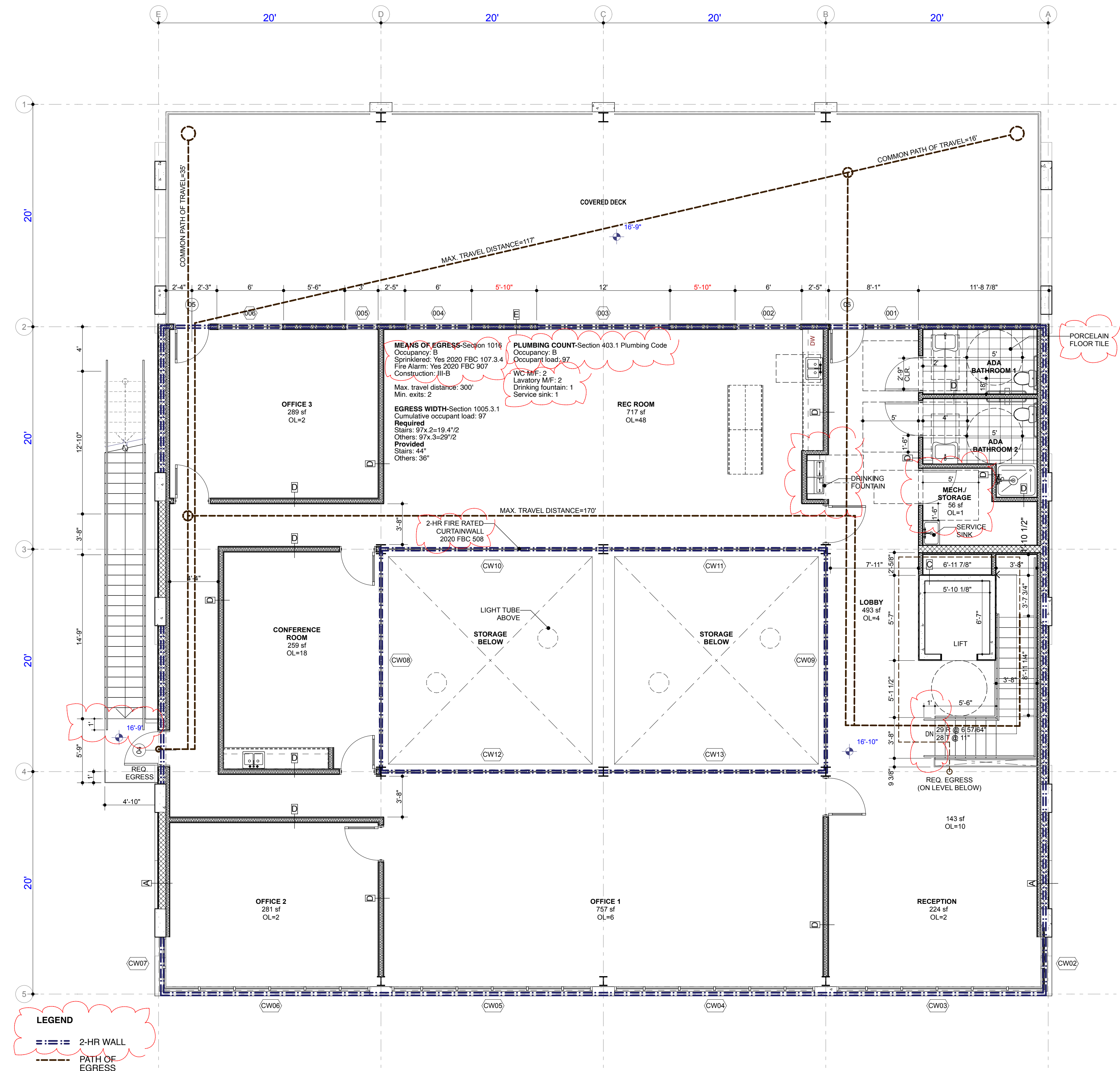
second level life safety plan scale: 3/16" = 1'-0"
