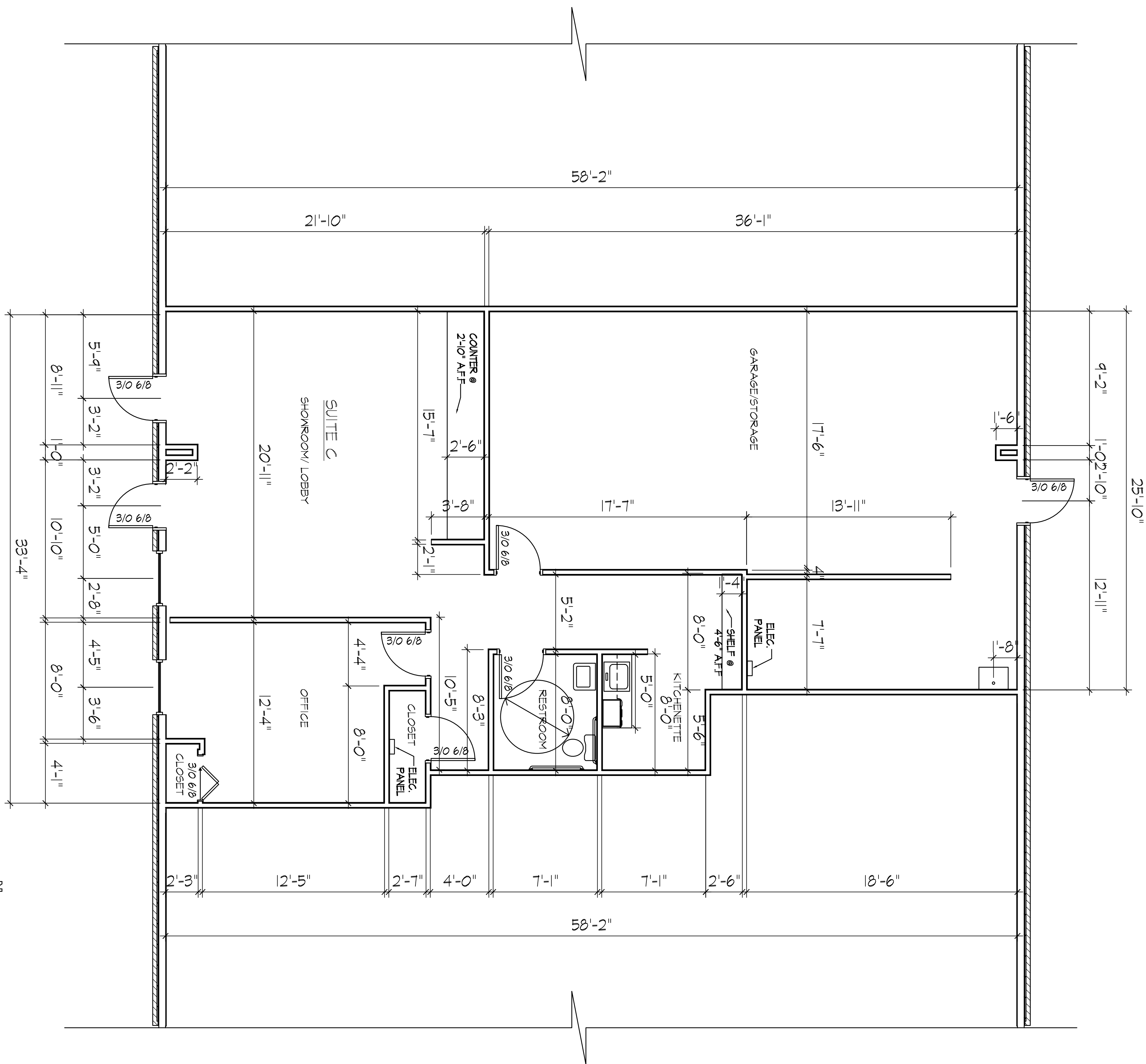
1 AS-BUILT FLOORPLAN SCALE: 1/4"=1'-0"
