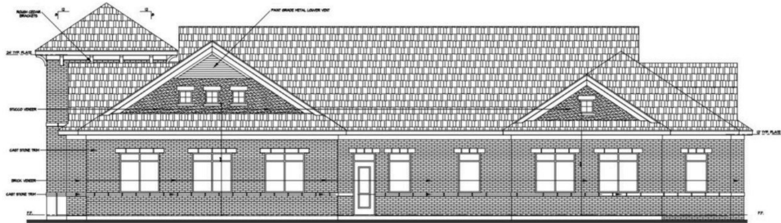
REAR (WEST) ELEVATION SCALE: 1/4\"/>
