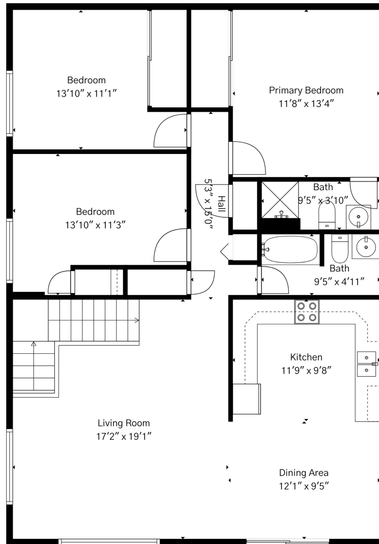
Floor 2
