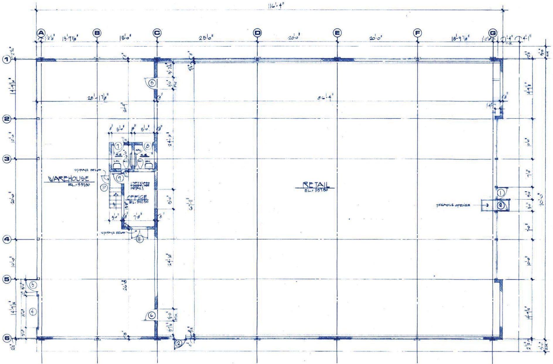
FLOOR PLAN 11/24/01
