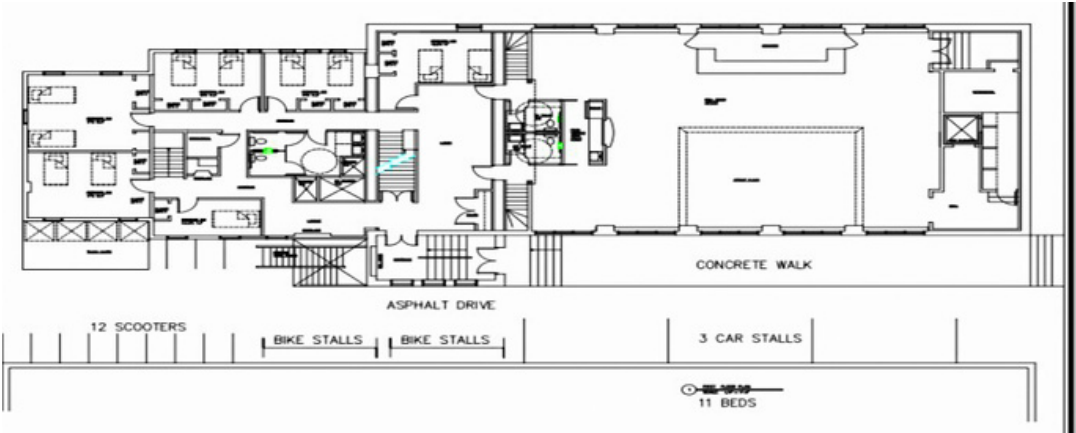
1st Floor
