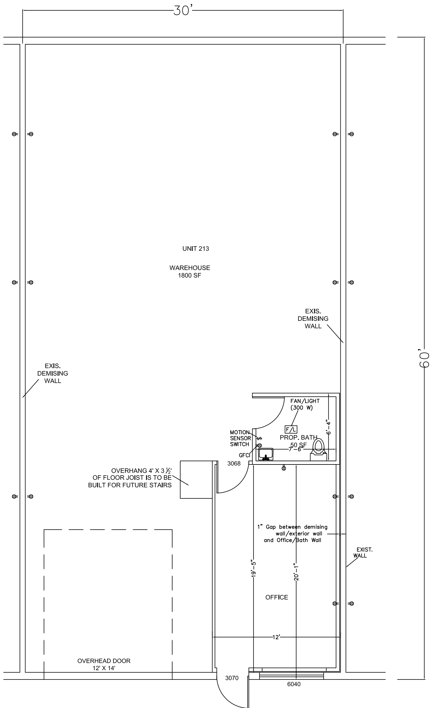
FLOOR PLAN
