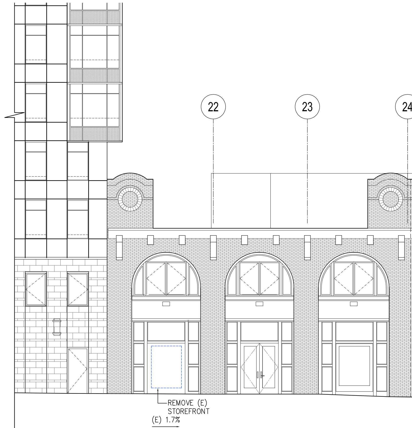
10 EXISTING ROSE STREET ELEVATION 1/8"=1'-0"
