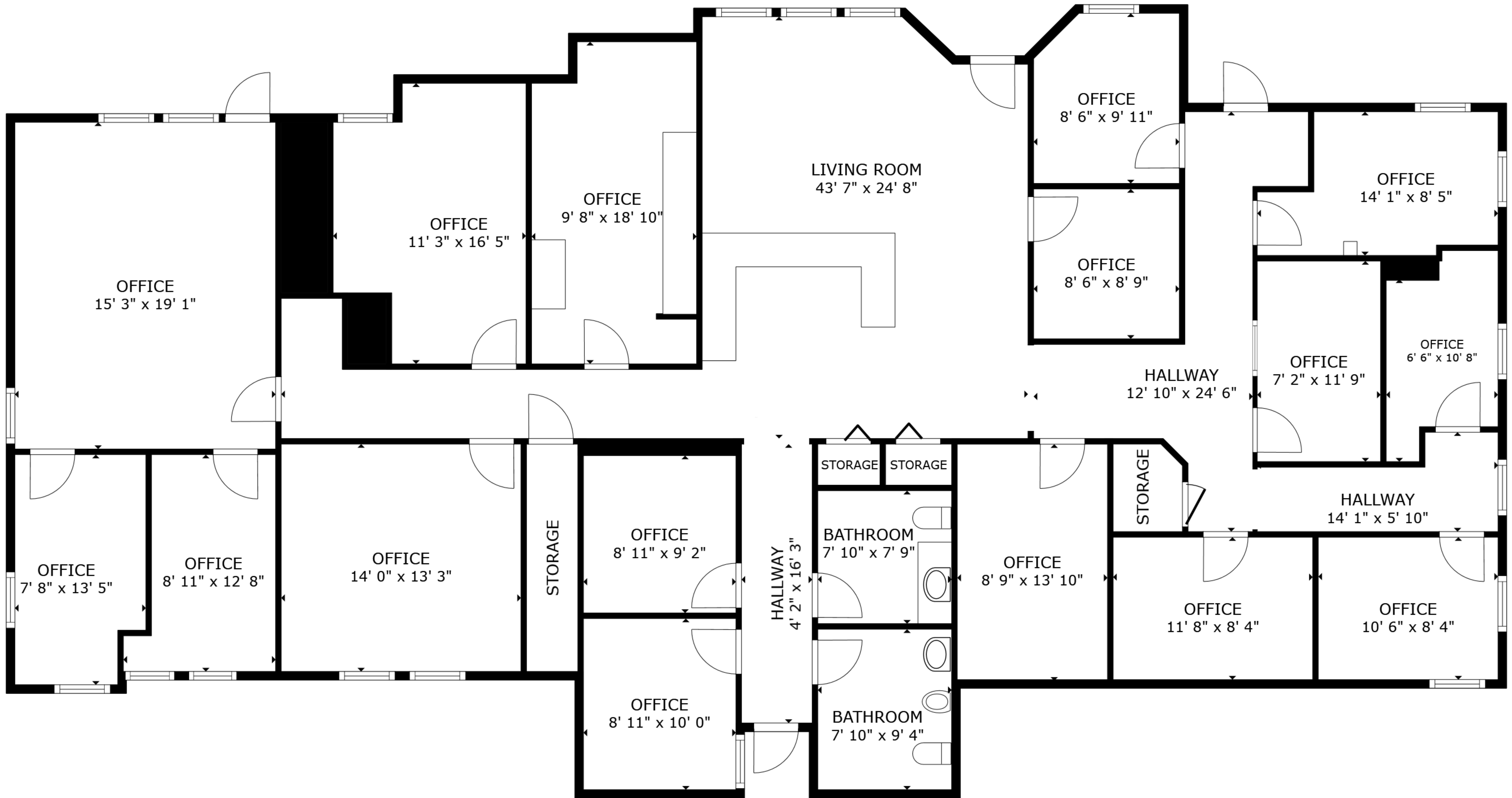
FLOOR PLAN
