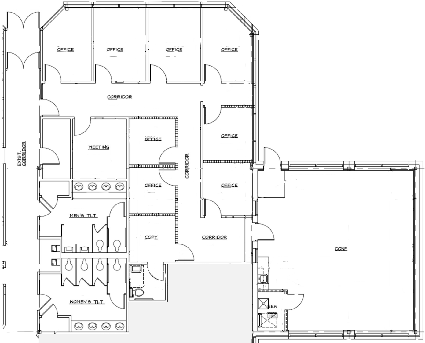
FLOOR PLAN 0 2' 4' 8' SCALE: 1/4" = 1'-0"
