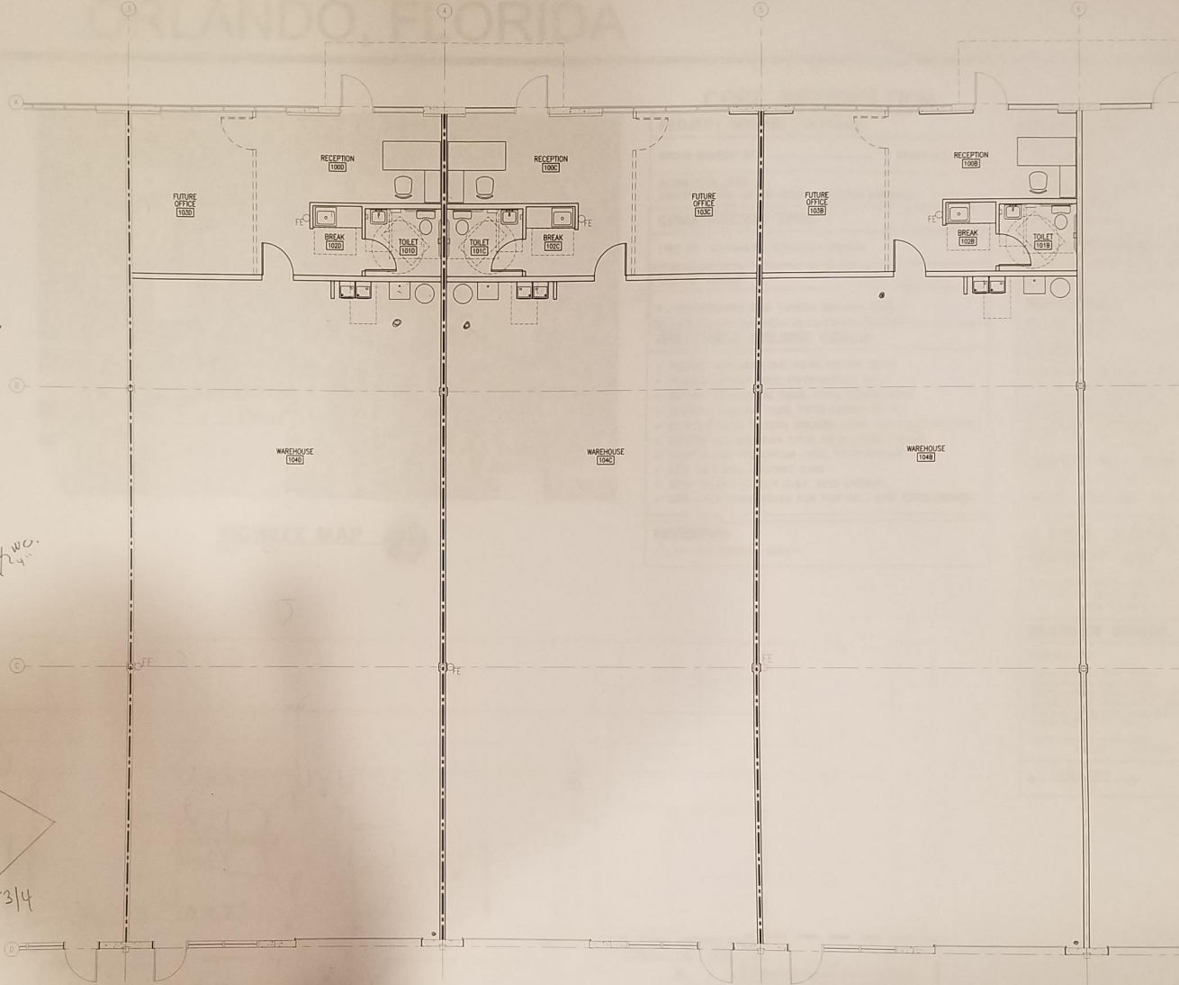
1 PLUMBING PLAN SCALE: 3/16" = 1'-0"
