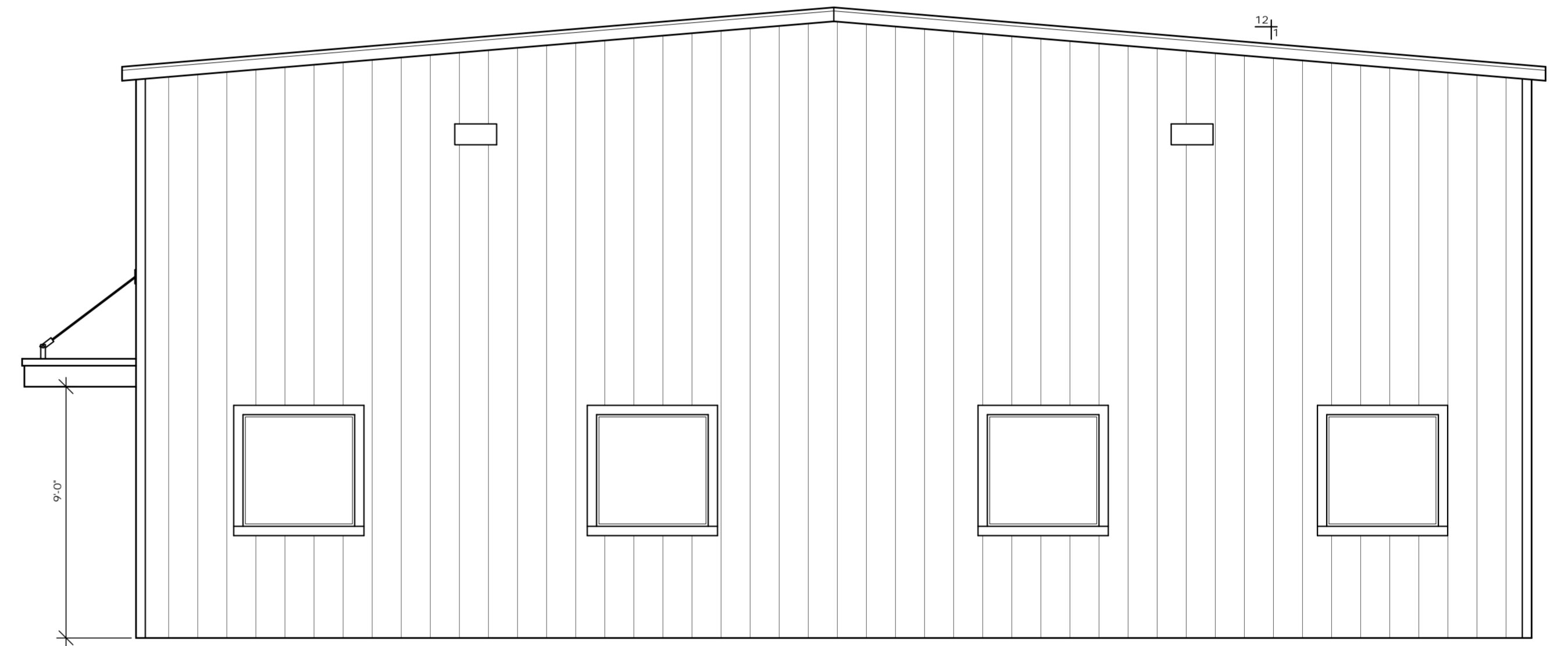
RIGHT SIDE ELEVATION SC: 1/4" = 1'-0"
