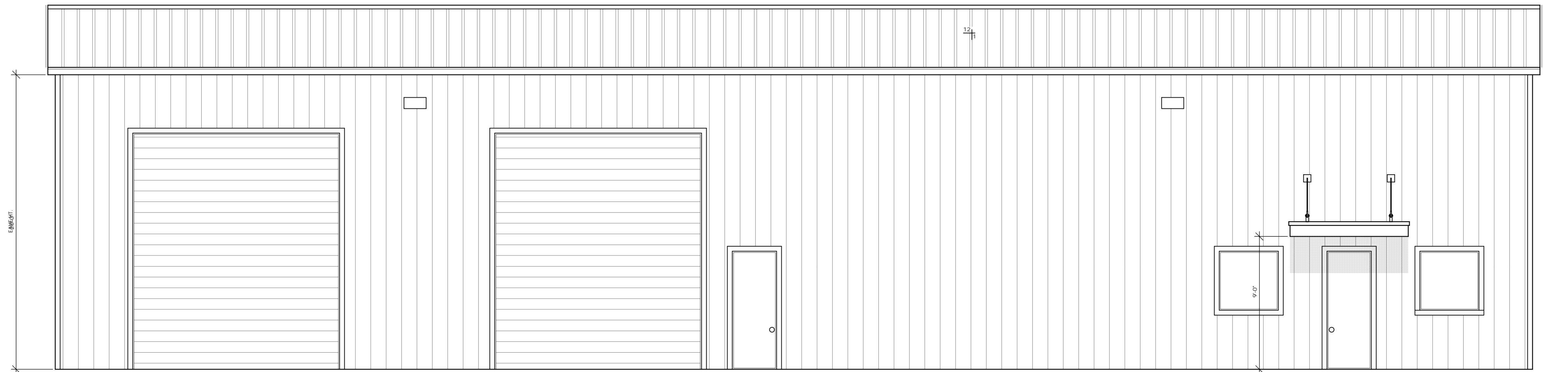
FRONT ELEVATION SC: 1/4" = 1'-0"
