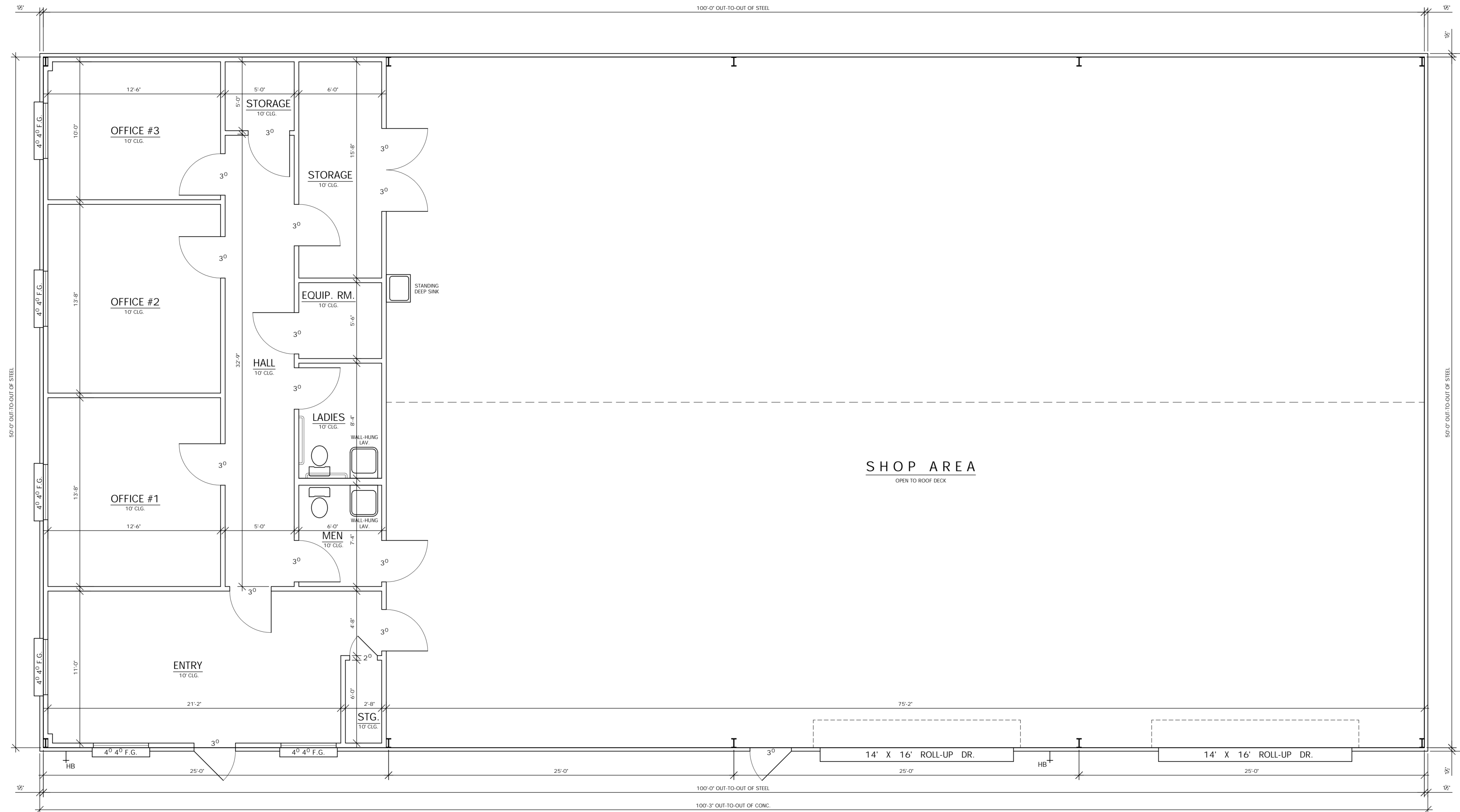
BLDG. 1 - FLOOR PLAN SC: 1/4" = 1'-0"
