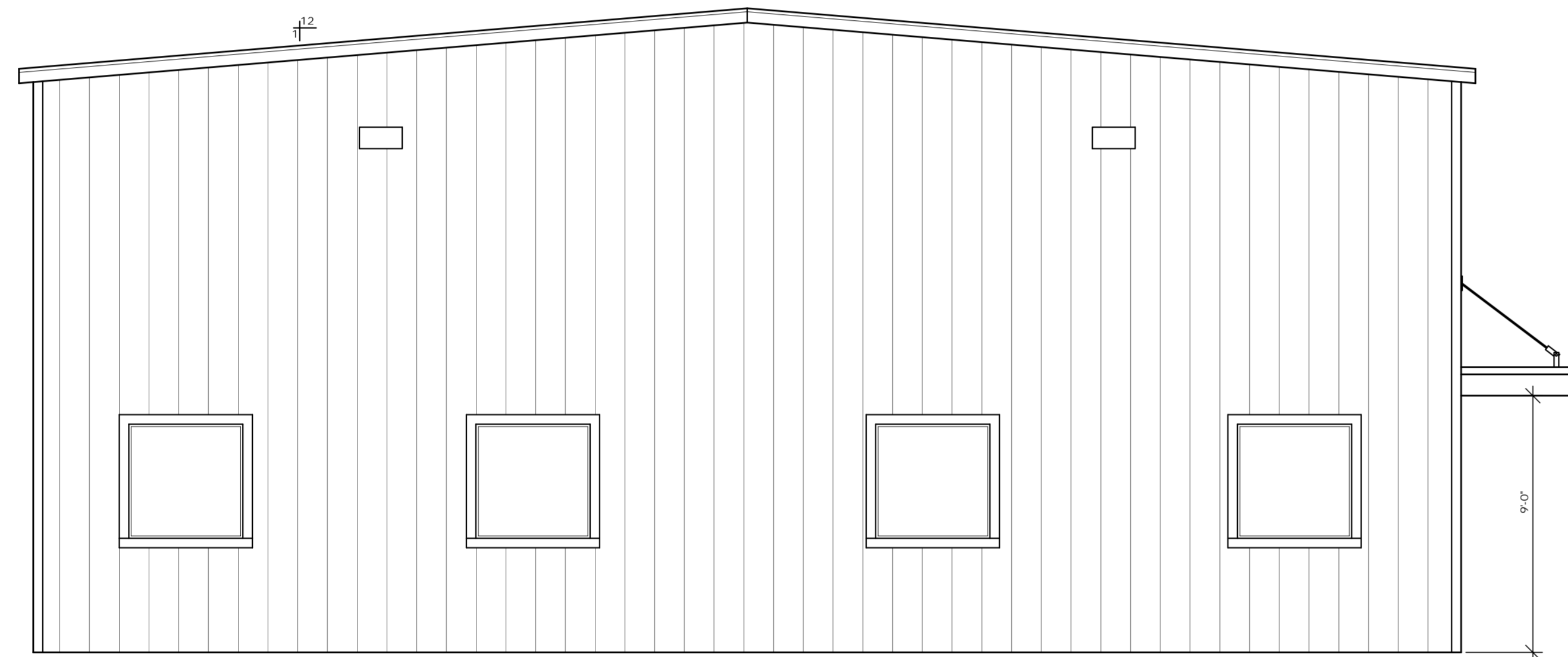
LEFT SIDE ELEVATION SC: 1/4" = 1'-0"
