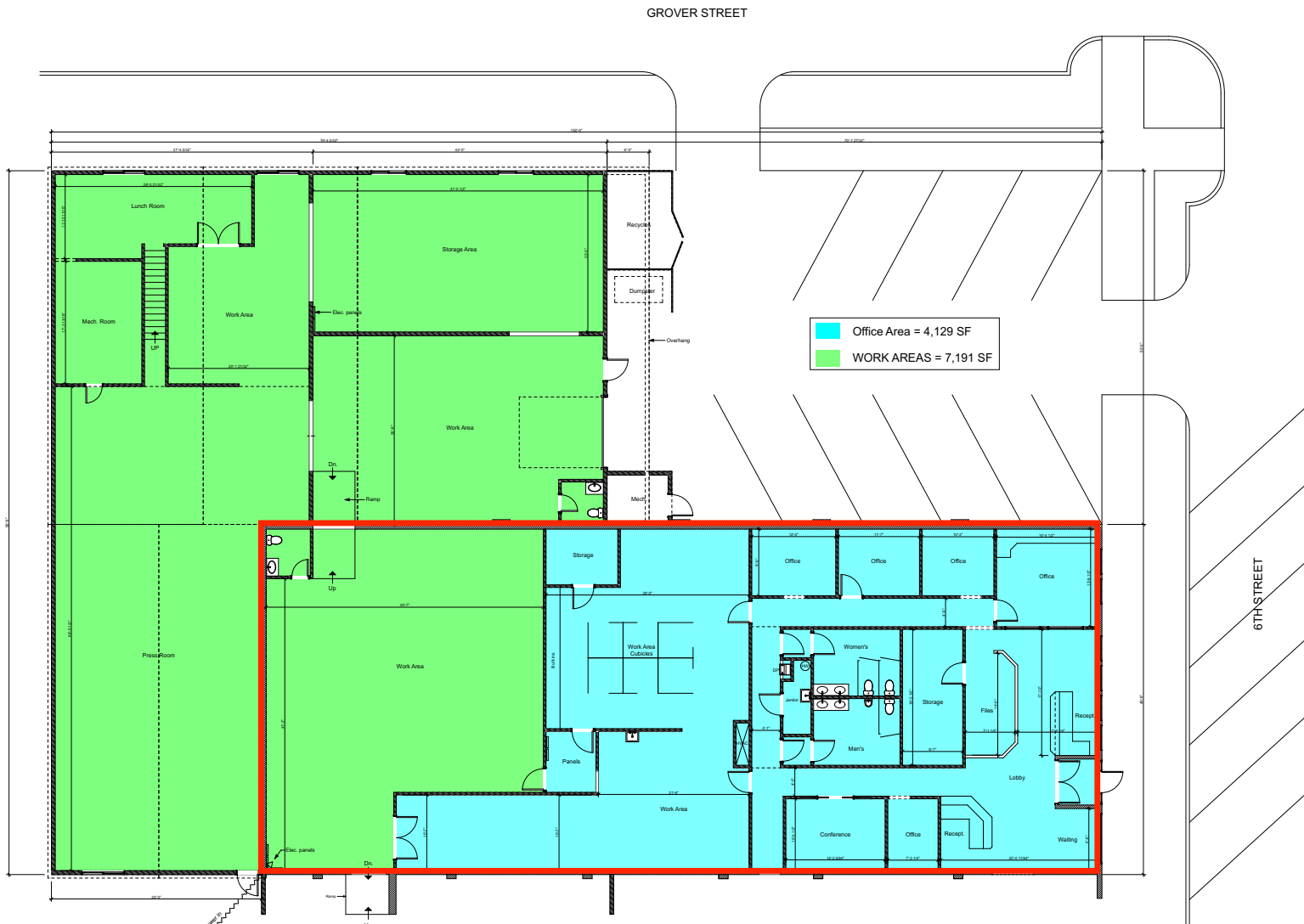
GROUND FLOOR PLAN - Existing 1/8" = 1' - 0"
