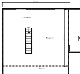
MEZZANINE 1/8" = 1' - 0"
