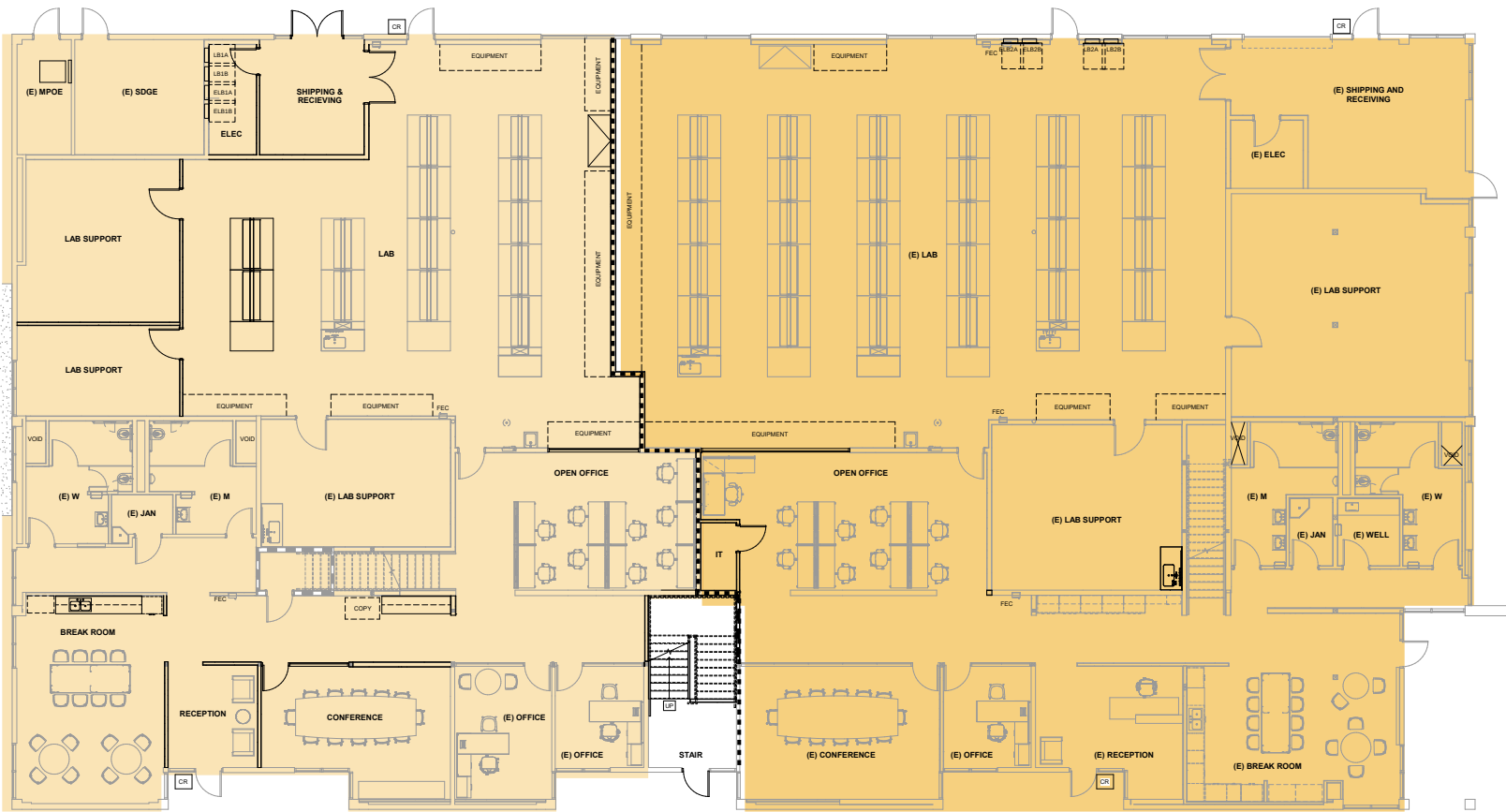
First Floor
