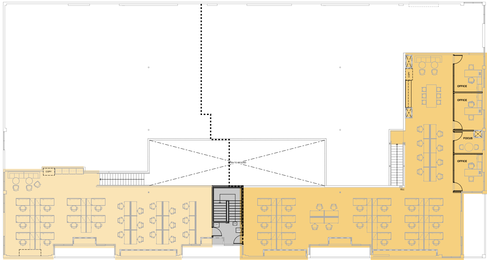
Second Floor
