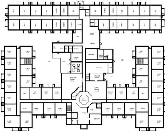
A1 Key Plan - First Floor A1.01 SCALE : 1/64" = 1'-0" REF:
