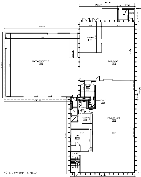
MAIN LEVEL
