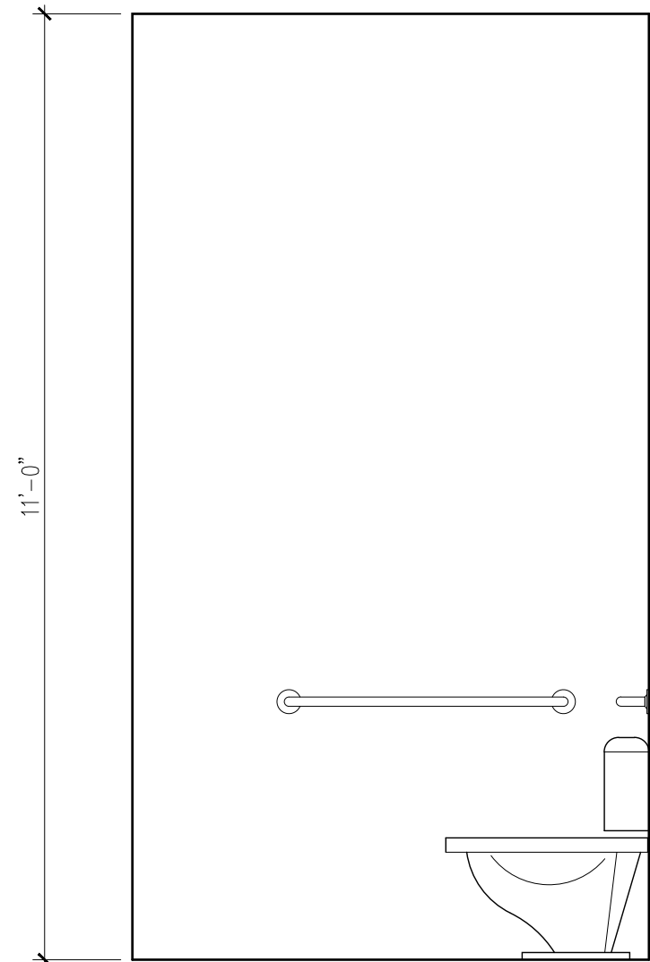
BATHROOM ELEVATION D
