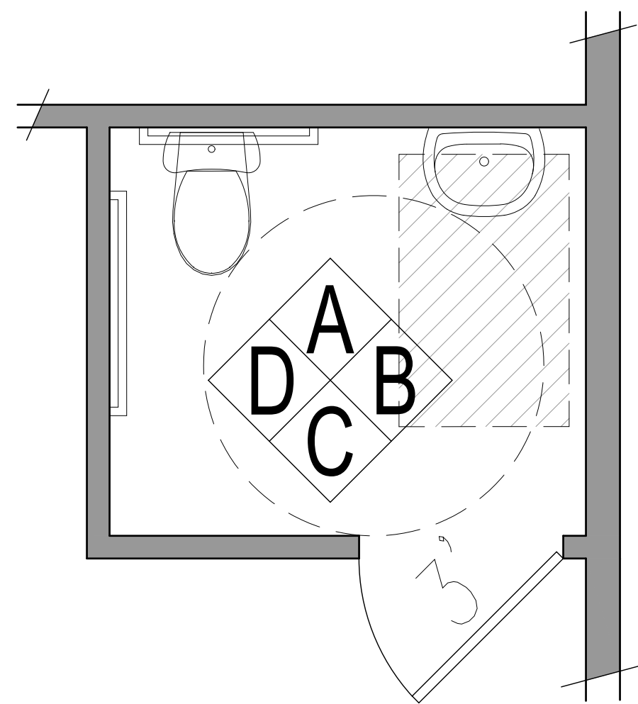
ADA BATHROOM PLAN
