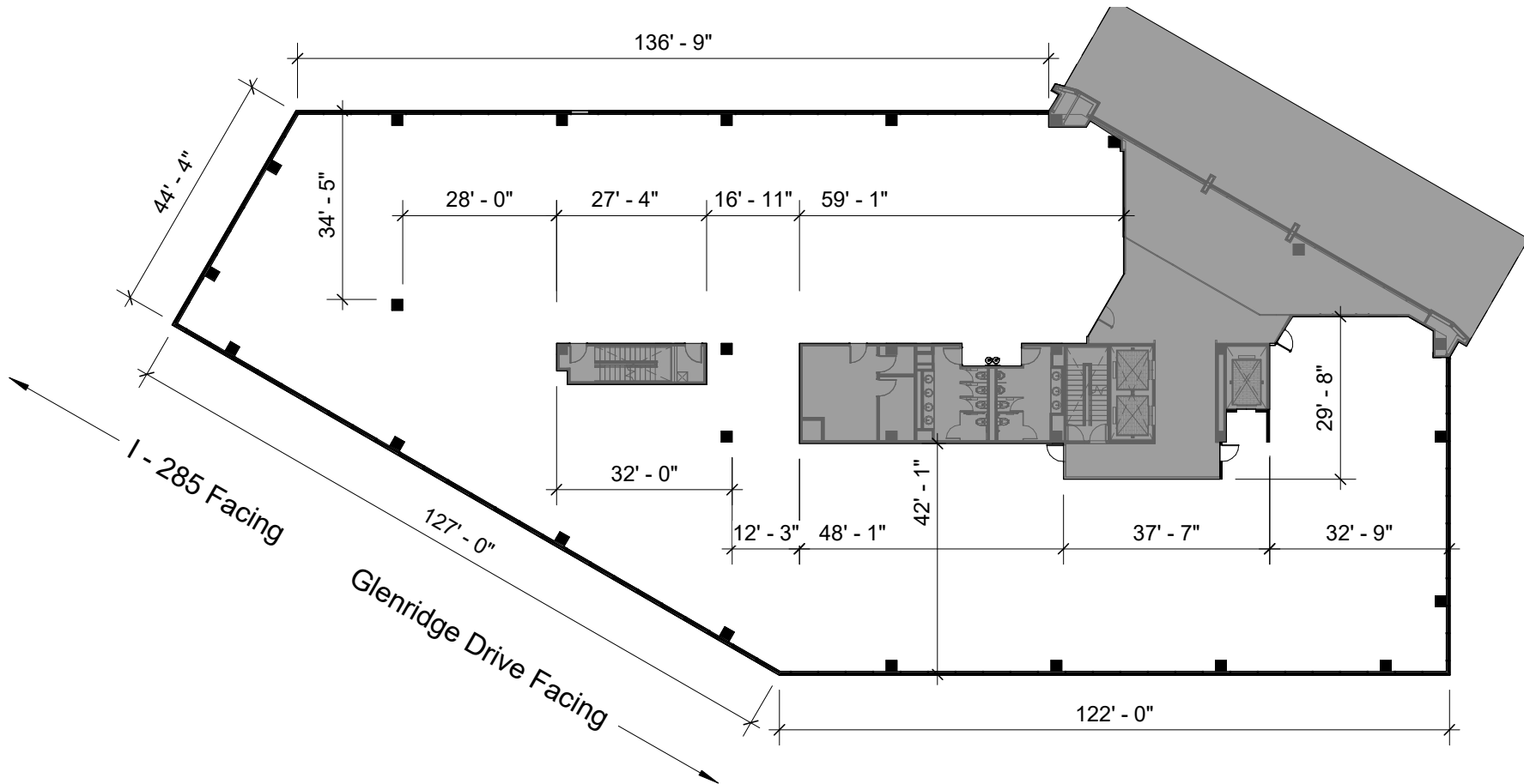
Floor Plan - Suite 200 West
