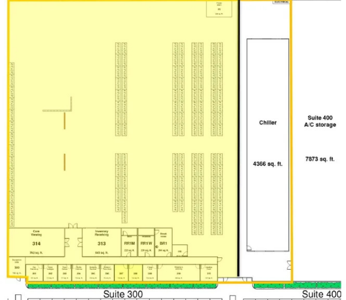
Floor Plan - Option B
