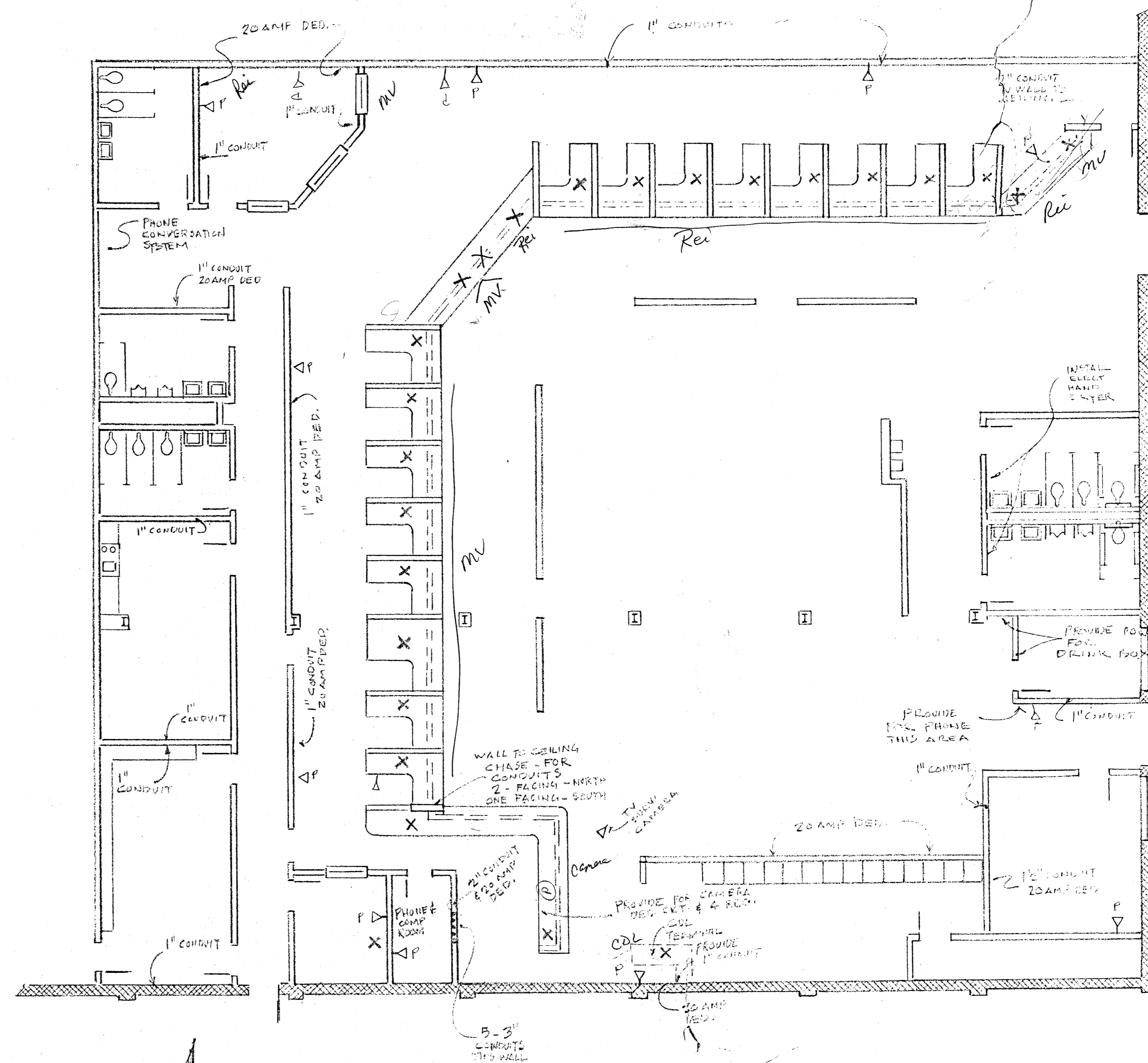
PLAN SHOWING ADDN POWER & CONDUITS TO BE INSTALLED
