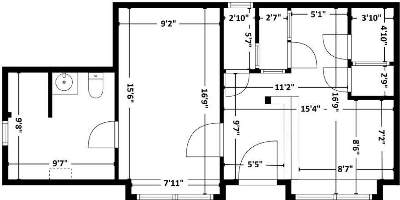
FLOOR PLAN
