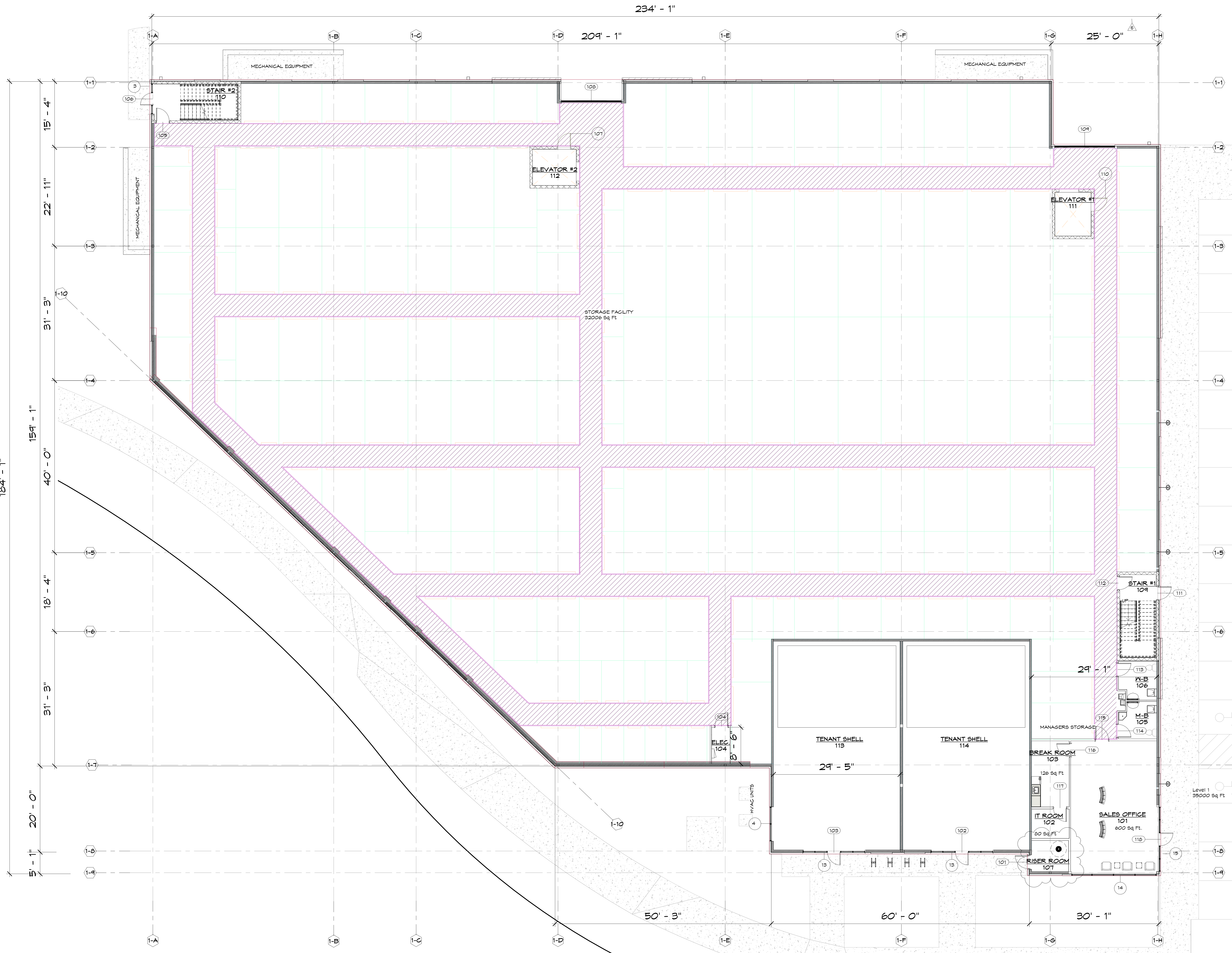
1 A-1.1 FIRST FLOOR PLAN SCALE 1/8" = 1'-0"
