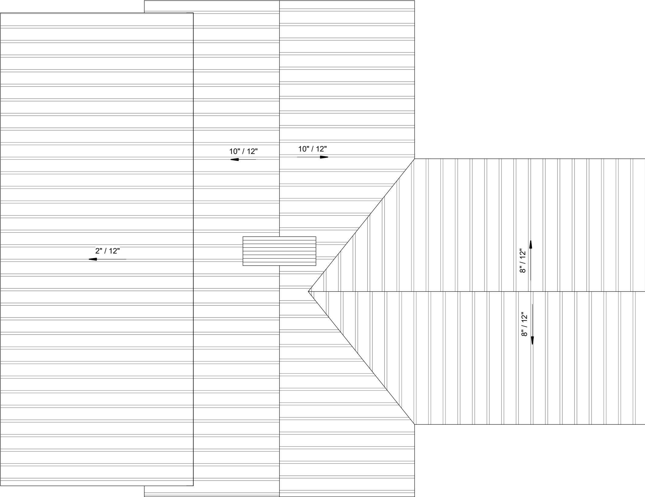
ROOF PLAN
