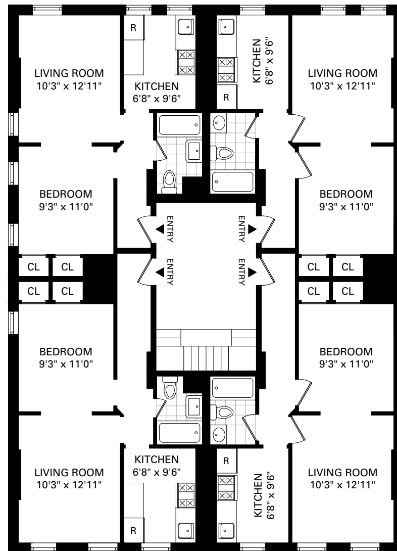
SECOND FLOOR
