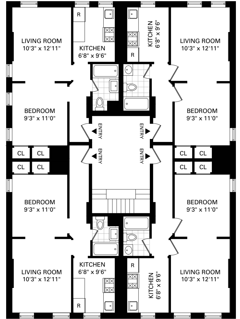
FOURTH FLOOR
