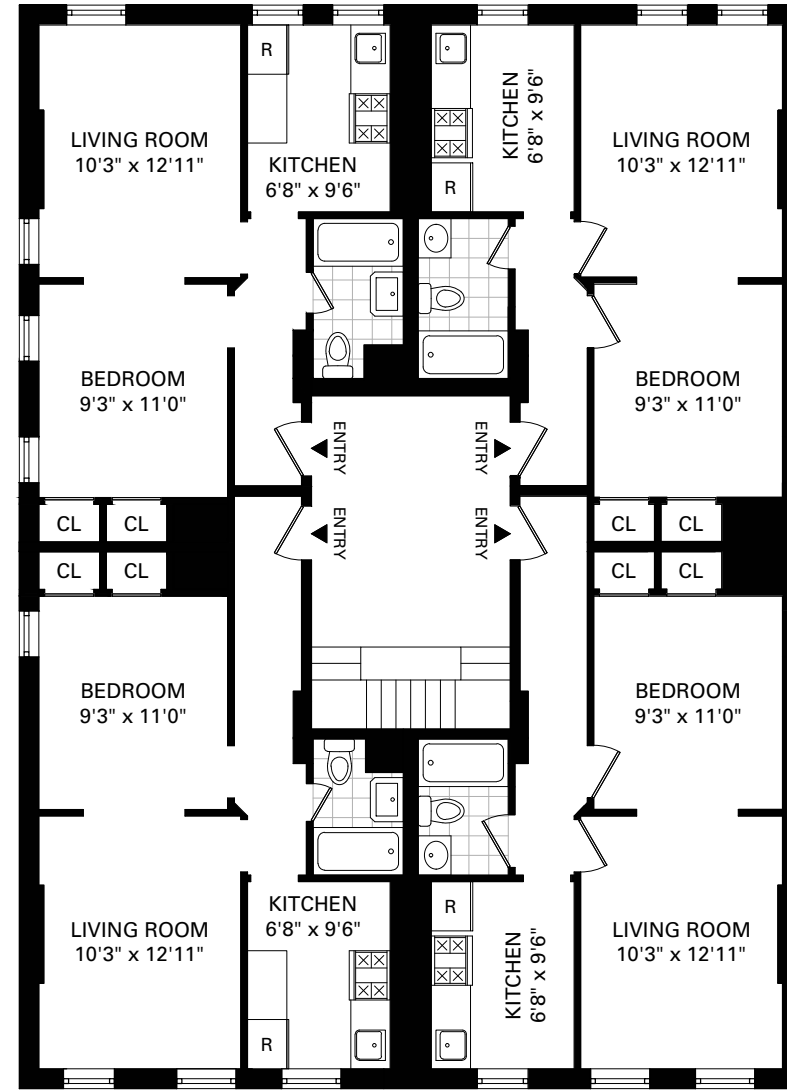
THIRD FLOOR
